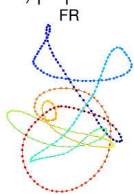
jagmesh1 ( |V| = 936, |E| = 2664 , sparsity = 0.609%) Figures are at 50 iterations.
