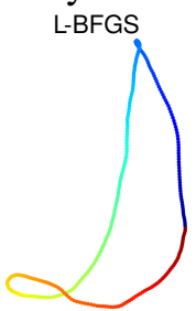
jagmesh1 ( |V| = 936, |E| = 2664 , sparsity = 0.609%) Figures are at 50 iterations.
