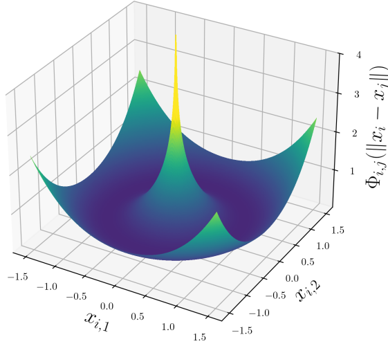
Figure 3: The energy \Phi_{i,j}(\|x_i - x_j\|) for x_i = (x_{i,1}, x_{i,2}) , x_j = (0, 0) , a_{i,j} = 1 , and k = 1 .
