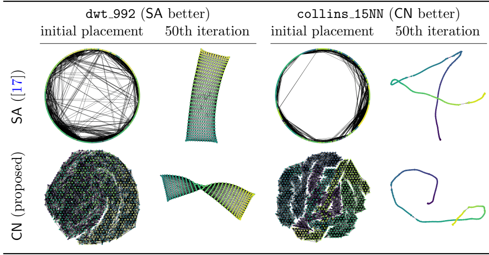
Figure 9: Visualization results showing initial and 50th iteration placements for dwt_992 and collins_15NN .
