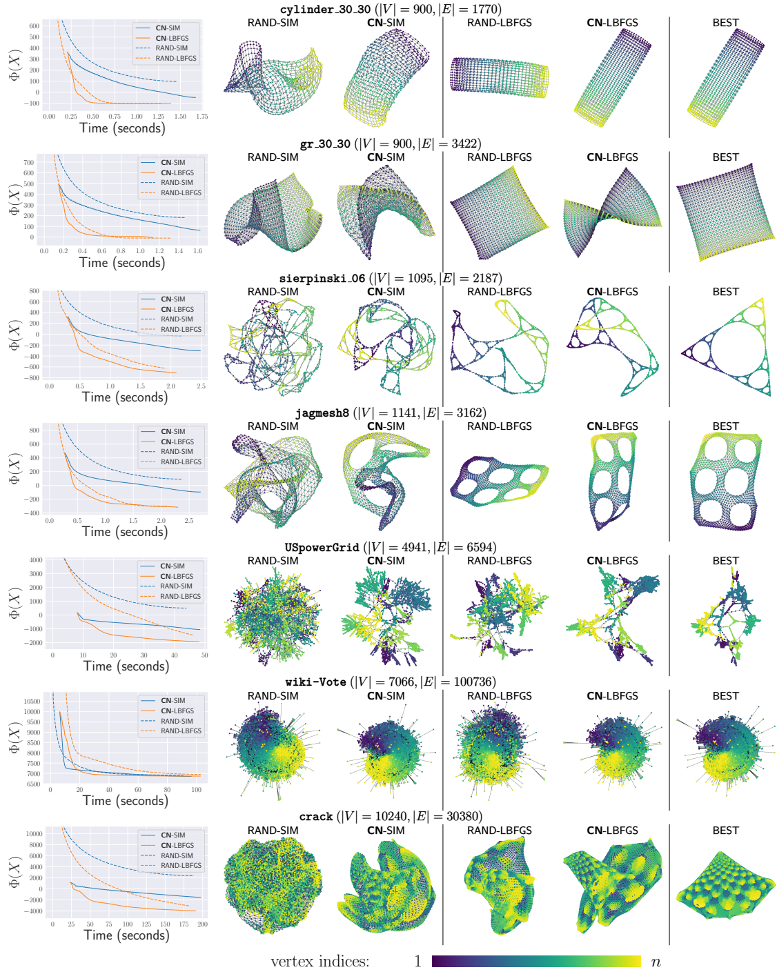
Figure 13: Additional experimental results for the FR force model. The objective function values at early states are generally improved for both simulation-based and L-BFGS algorithms, and the visual improvements by our proposed method CN are apparent for the simulation-based algorithms.
