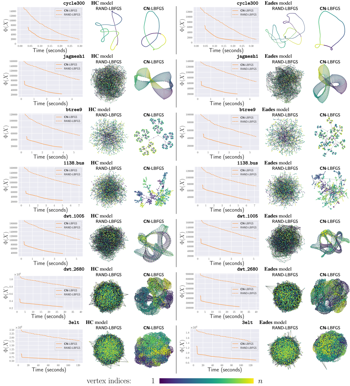
Figure 7: Experimental results for the HC and Eades force models. Our proposed method CN yields improved results.
