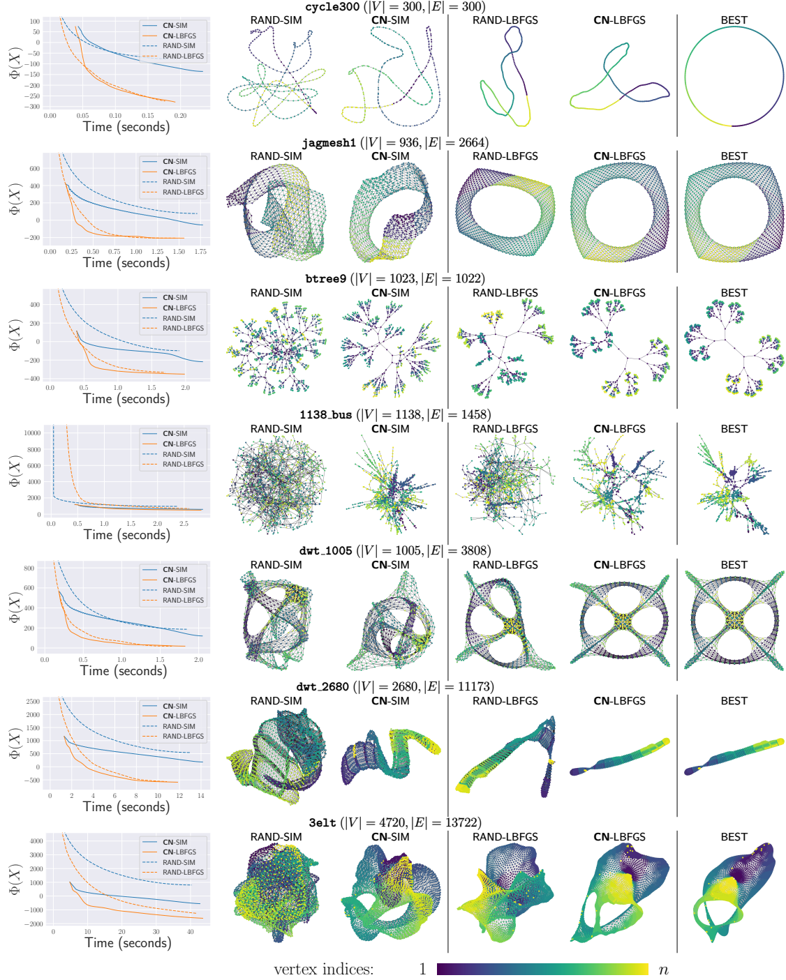
Figure 6: Experimental results for the FR force model. Our proposed method CN yields improved results for both the simulation-based algorithm and L-BFGS.
