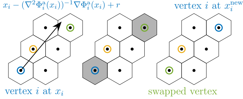
Figure 5: One iteration of the proposed algorithm. Step 1. Compute the coordinate Newton direction (blue). Step 2. Decide x_i^{\text{new}} by adding a random vector and rounding. Step 3. Move the vertex and swap the vertices if necessary (swap blue and green vertices).
