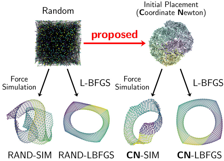
Figure 1: Comparison of the algorithms for the jagmesh1 .
