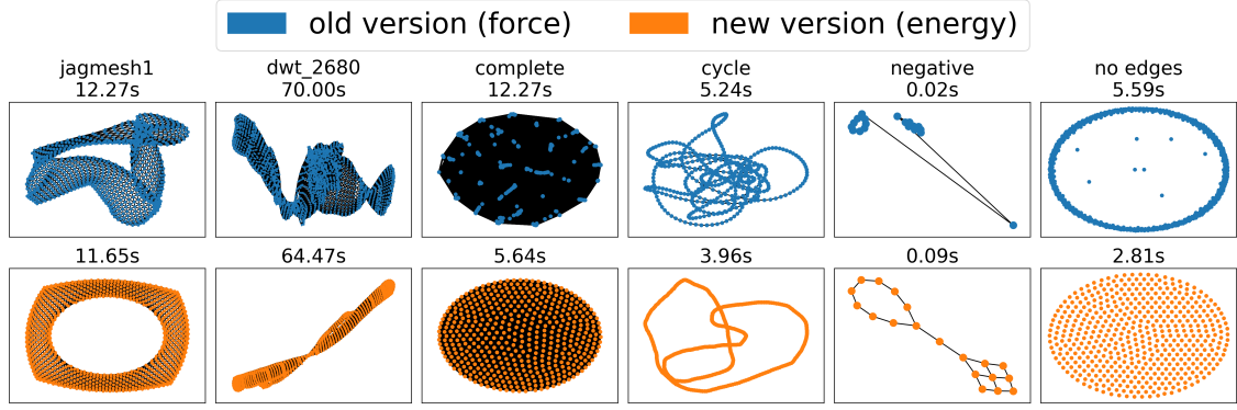
Figure 15: The simulation-based (FR) algorithm and L-BFGS algorithm in NetworkX.
