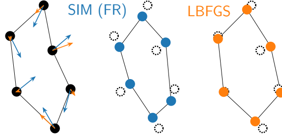
Figure 14: Comparison of the simulation-based and L-BFGS algorithms. Blue arrows represent fixed stepsizes in FR, whereas orange arrows represent adaptive stepsizes determined by the approximate inverse Hessian.
