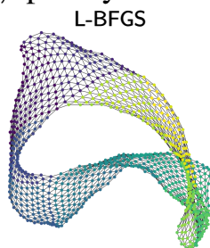
dwt_1005 ( |V| = 1005, |E| = 3808 , sparsity = 0.755%) Figures are at 100 iterations.
