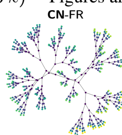
1138_bus ( |V| = 1138, |E| = 1458 , sparsity = 0.225%) Figures are at 150 iterations.
