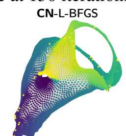
3elt ( |V| = 4720, |E| = 13722 , sparsity = 0.123%) Figures are at 150 iterations.
