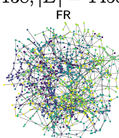
dwt_2680 ( |V| = 2680, |E| = 11173 , sparsity = 0.311%) Figures are at 150 iterations.
