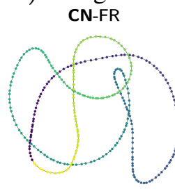
jagmesh1 ( |V| = 936, |E| = 2664 , sparsity = 0.609%) Figures are at 50 iterations.
