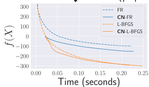
jagmesh1 ( |V| = 936, |E| = 2664 , sparsity = 0.609%) Figures are at 50 iterations.
