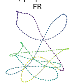
jagmesh1 ( |V| = 936, |E| = 2664 , sparsity = 0.609%) Figures are at 50 iterations.
