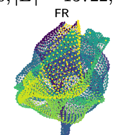
3elt ( |V| = 4720, |E| = 13722 , sparsity = 0.123%) Figures are at 150 iterations.
