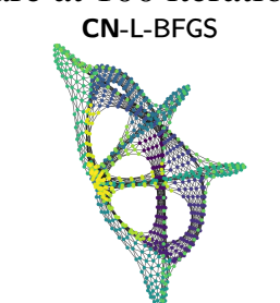
btrees9 ( |V| = 1023, |E| = 1022 , sparsity = 0.196%) Figures are at 150 iterations.
