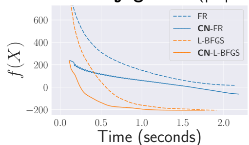
dwt_1005 ( |V| = 1005, |E| = 3808 , sparsity = 0.755%) Figures are at 100 iterations.
