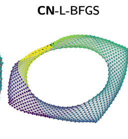
dwt_1005 ( |V| = 1005, |E| = 3808 , sparsity = 0.755%) Figures are at 100 iterations.
