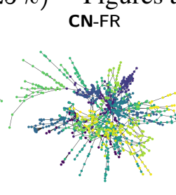
dwt_2680 ( |V| = 2680, |E| = 11173 , sparsity = 0.311%) Figures are at 150 iterations.
