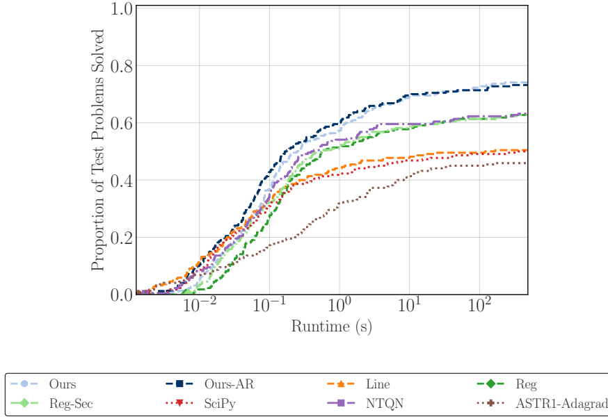
Fig. 6: Time-to-solution comparison with 32-bit evaluations and \epsilon_{\text{gtol}} = 10^{-3} . Each curve shows the fraction of problems reaching the gradient tolerance within the elapsed time.
