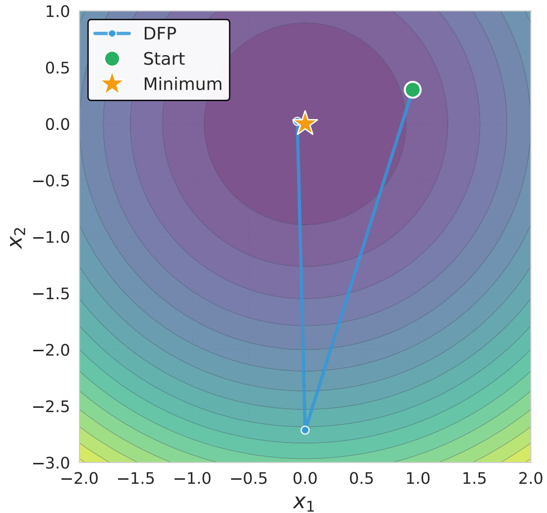
DFP Trajectory ( \lambda=0.1 )
