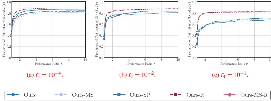
Fig. 2: Performance profile for the deliberately adverse joint function-and-gradient noise setting (componentwise level 10^{-3} ) and \varepsilon_{\text{gtol}} = 10^{-2} . This experiment lies outside the exact-gradient theory.
