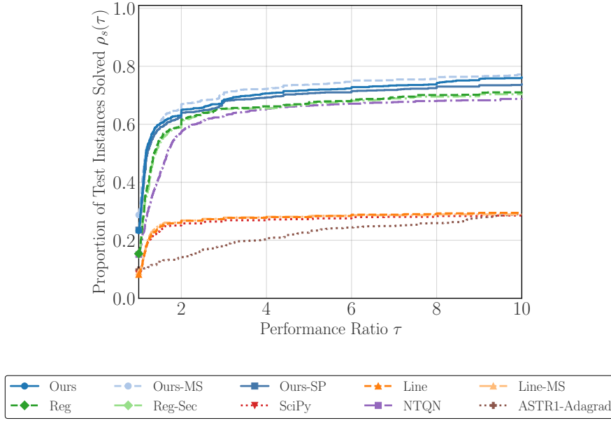
Fig. 2: Performance profile for the deliberately adverse joint function-and-gradient noise setting (componentwise level 10^{-3} ) and \varepsilon_{\text{gtol}} = 10^{-2} . This experiment lies outside the exact-gradient theory.
