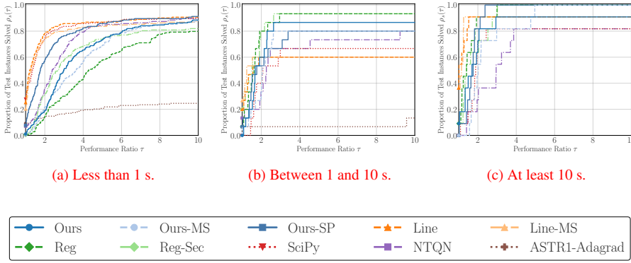
Fig. 6: Performance profiles for the 64-bit setting at \epsilon_{\text{gtol}} = 10^{-3} , grouped by the best runtime attained by any method on each problem instance.
