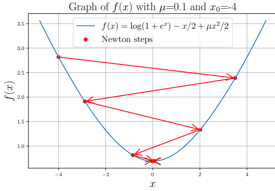
Figure 4: (Left) Newton's method converges for x_0 = -4 , \mu = 0.1 . (Right) Newton's method oscillates for x_0 = -4 , \mu = 0.01 .
