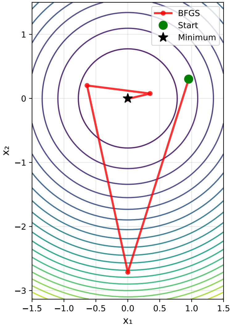
BFGS Trajectory (lambda=0.1)
