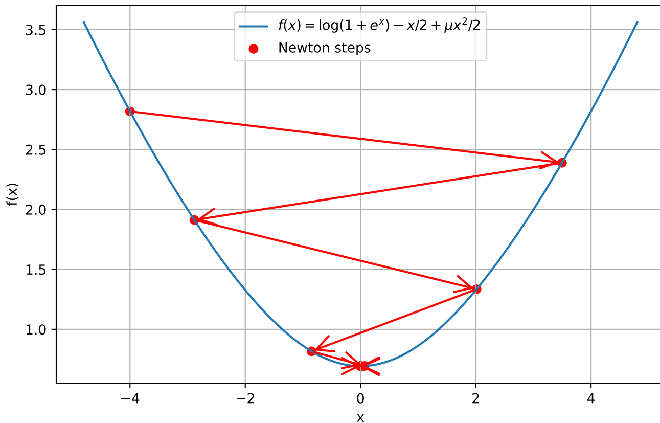
Graph of f(x) with \mu=0.1 and x_0=-4
