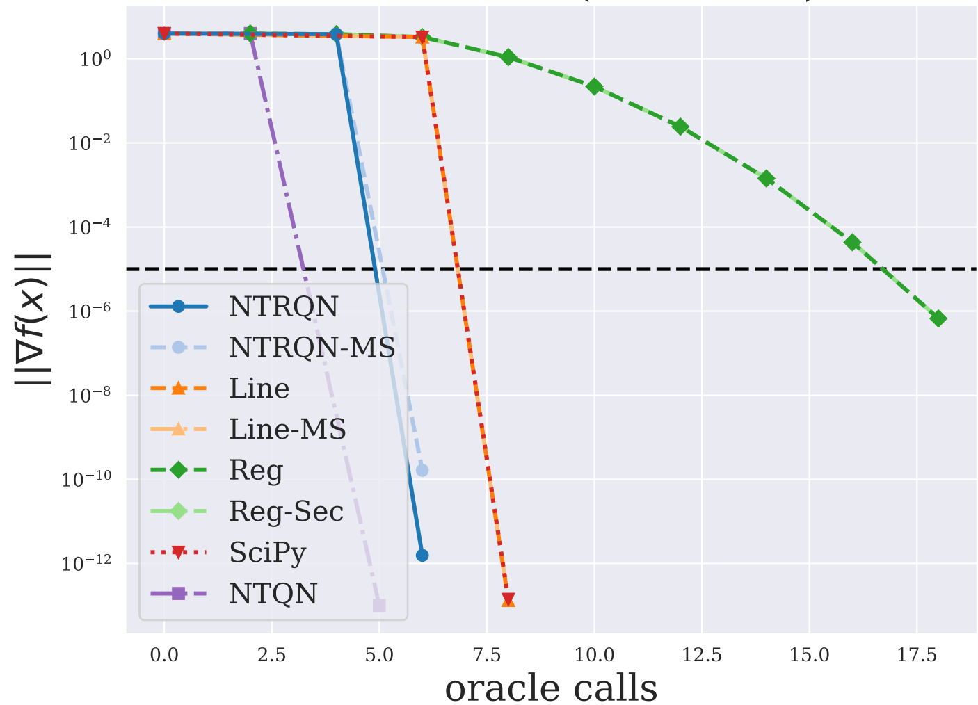
ARGLINA ( n = 200 )
