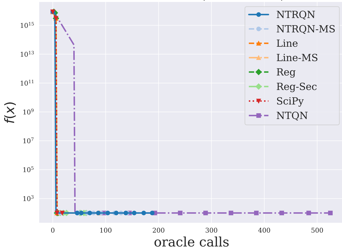
ARGLINB ( n = 200 )
