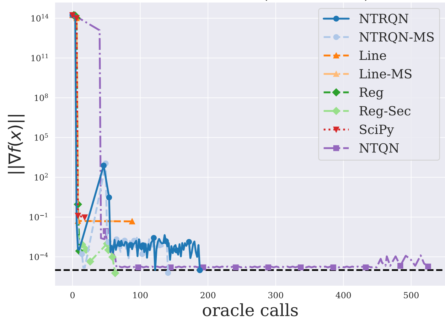
ARGLINB ( n = 200 )
