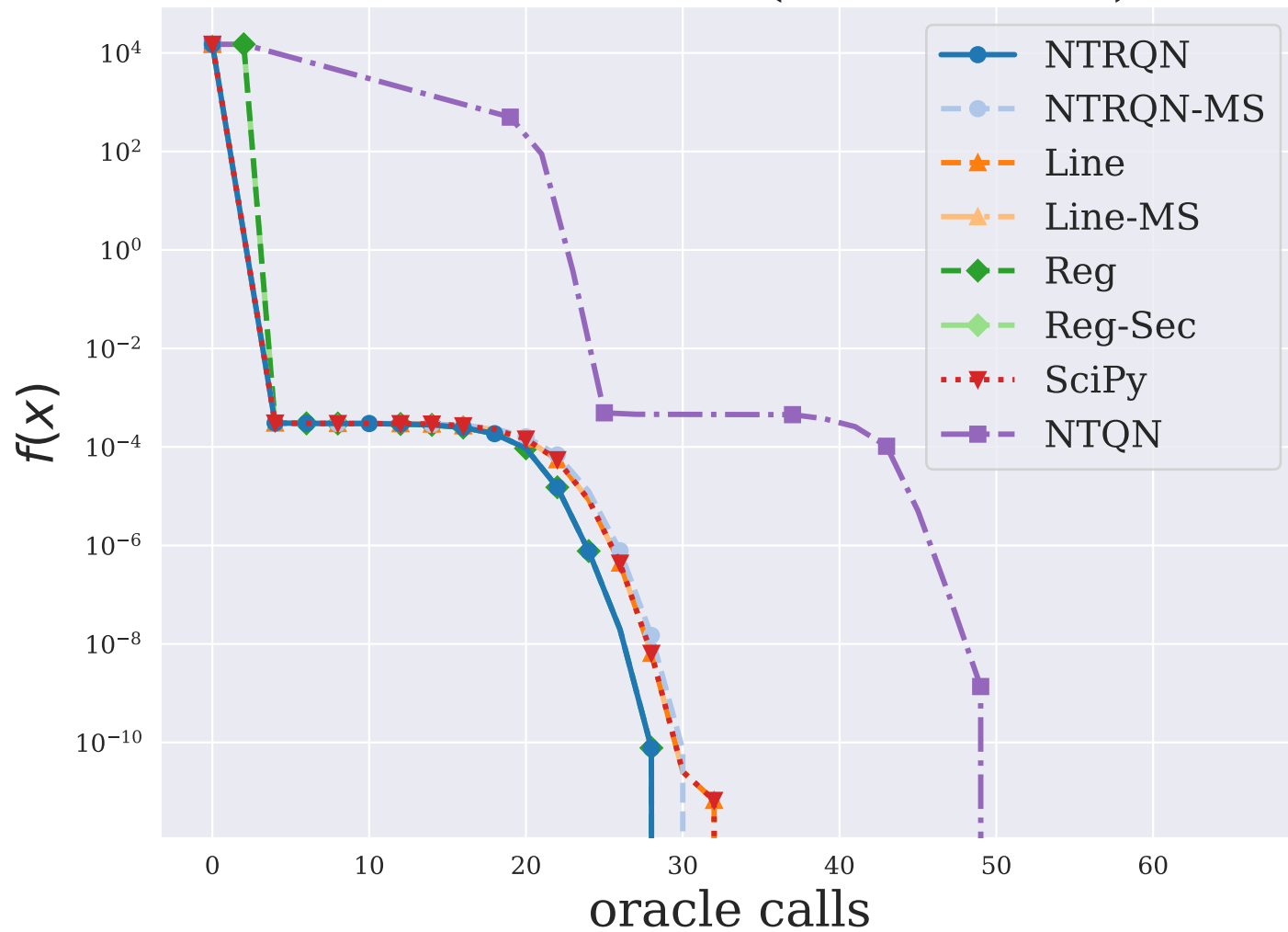
ARWHEAD ( n = 5000 )
