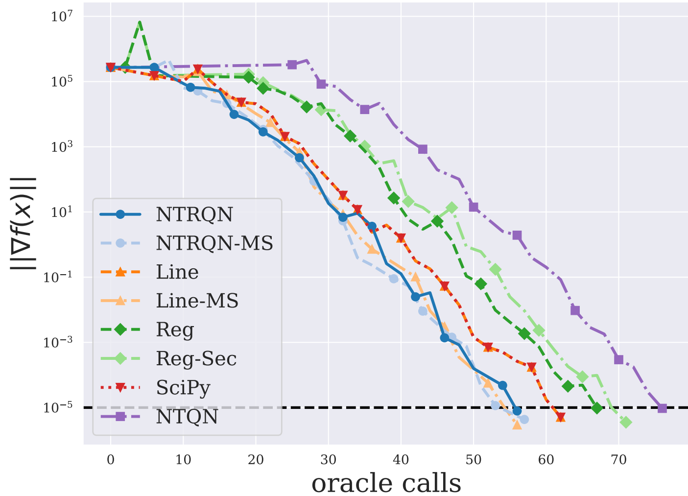
BA-L1SPLS ( n = 57 )
