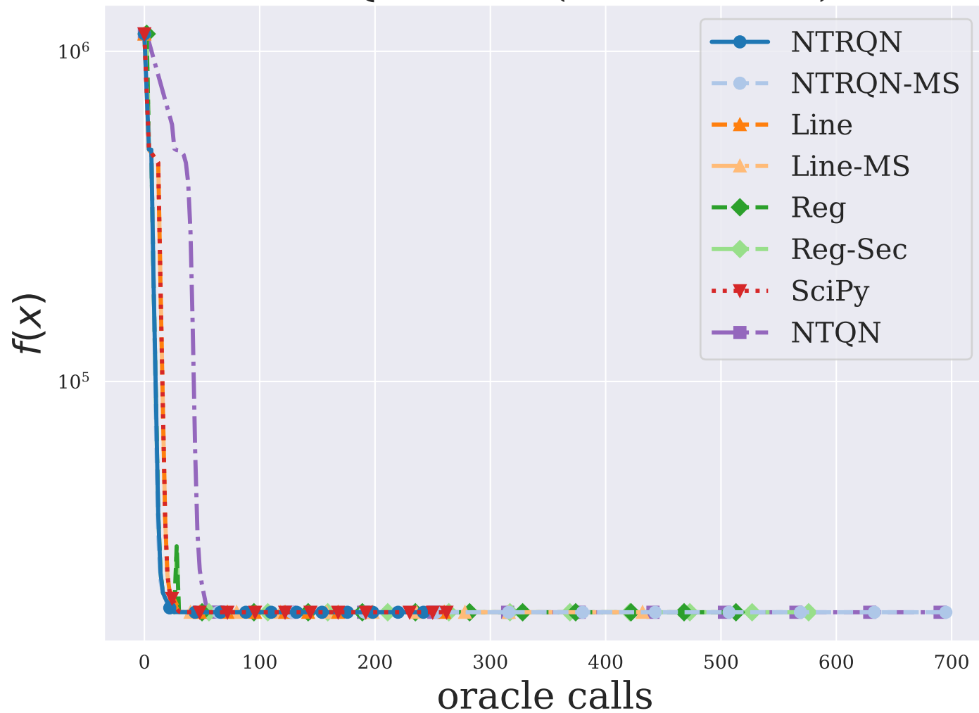
BDQRTIC ( n = 5000 )
