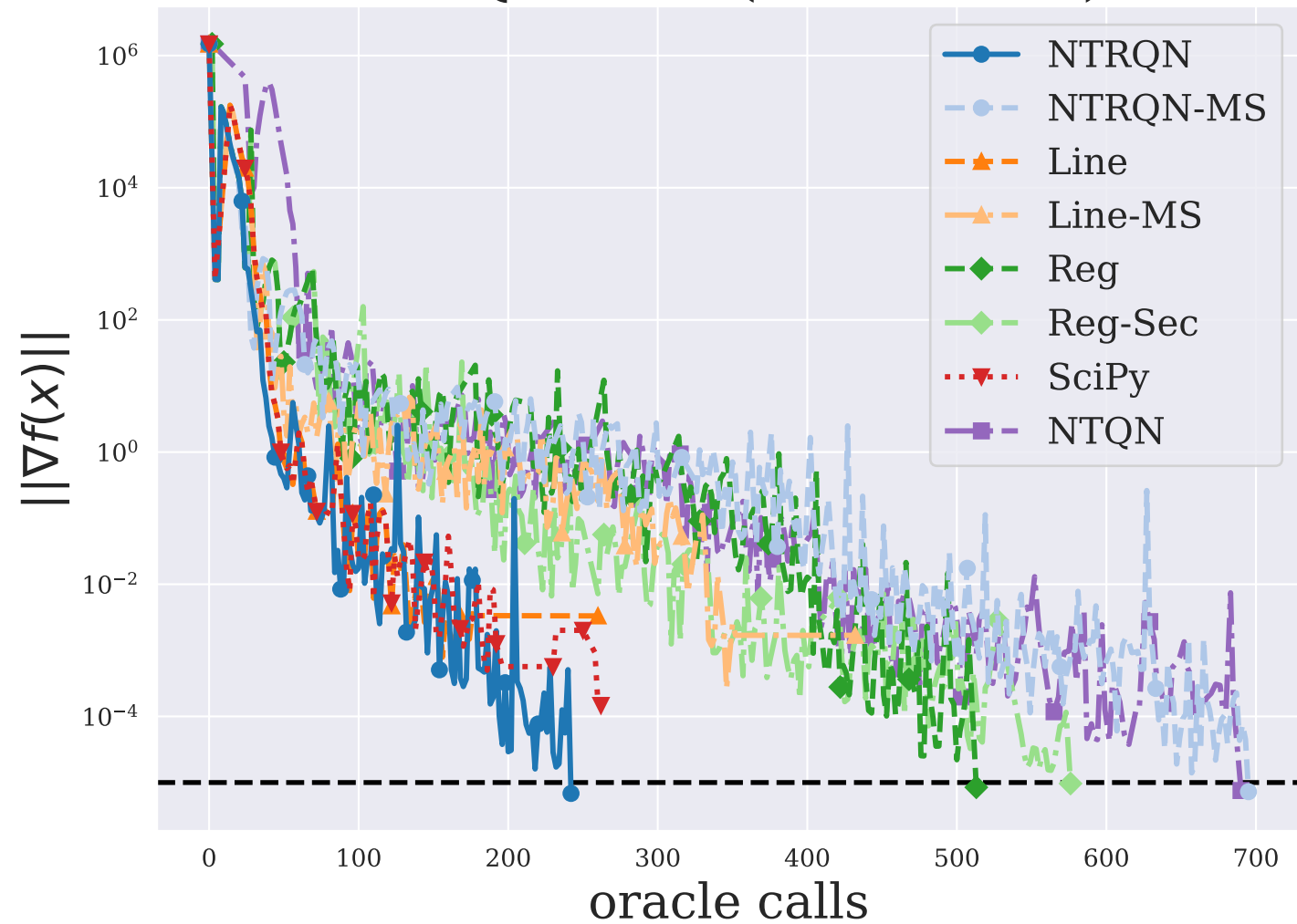
BDQRTIC ( n = 5000 )
