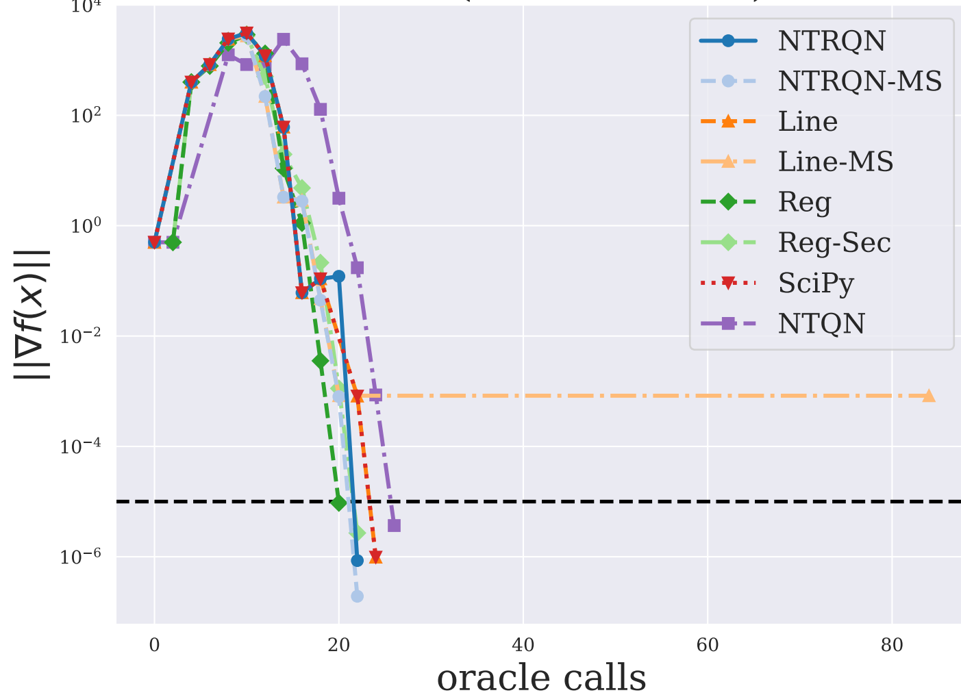
BOX ( n = 10000 )
