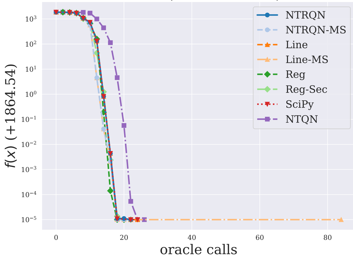
BOX ( n = 10000 )
