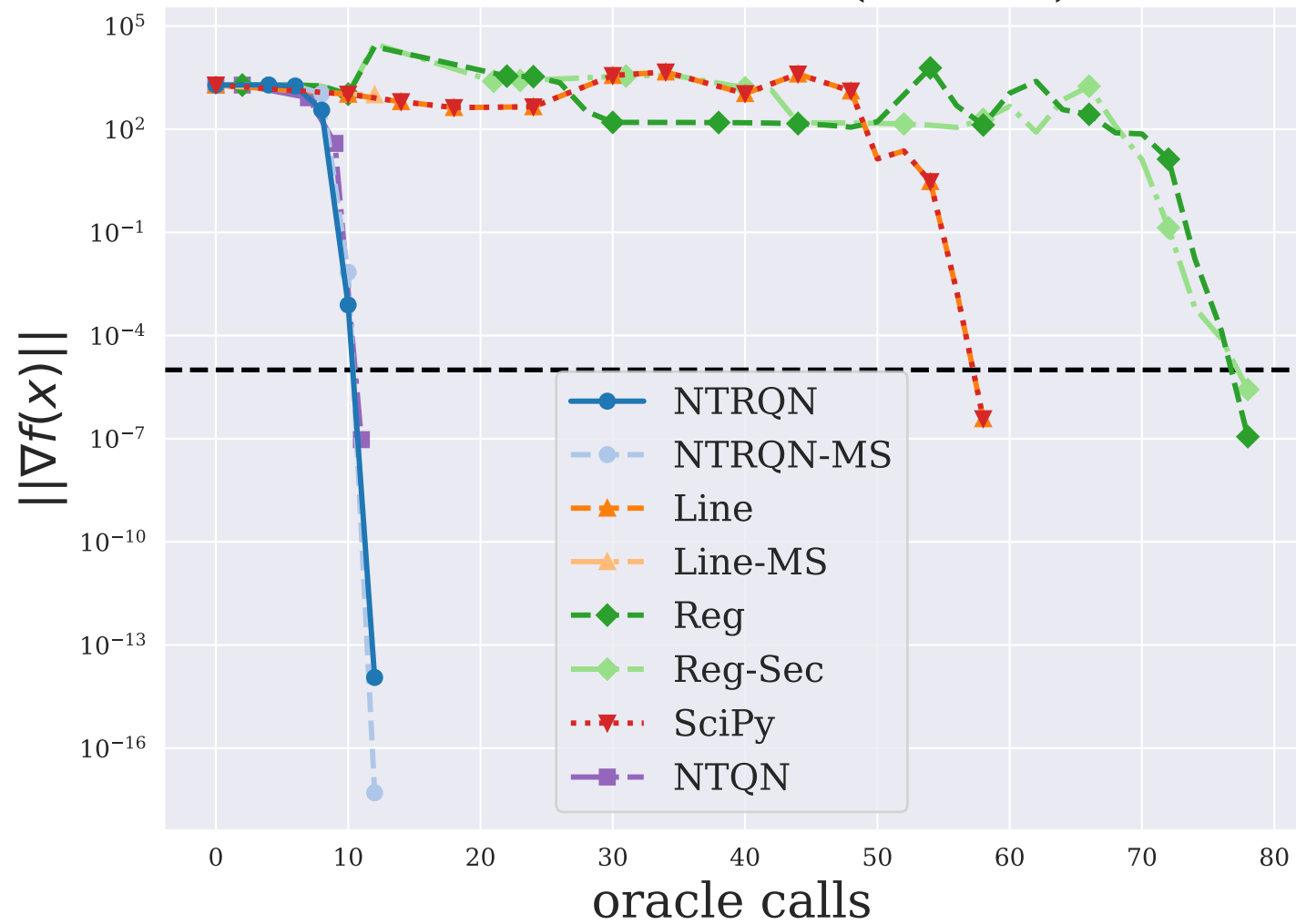
BOXBODLS ( n = 2 )
