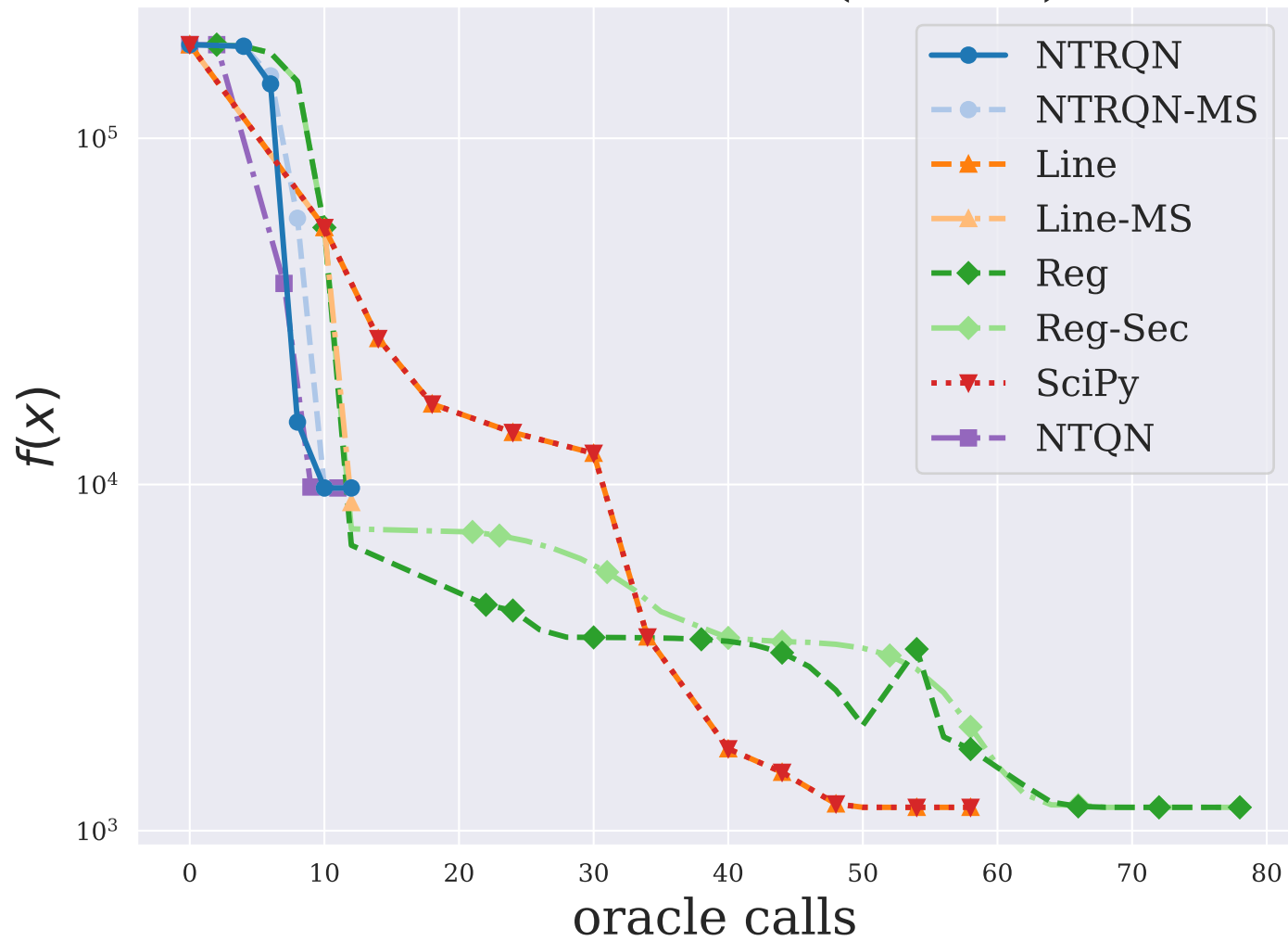
BOXBODLS ( n = 2 )
