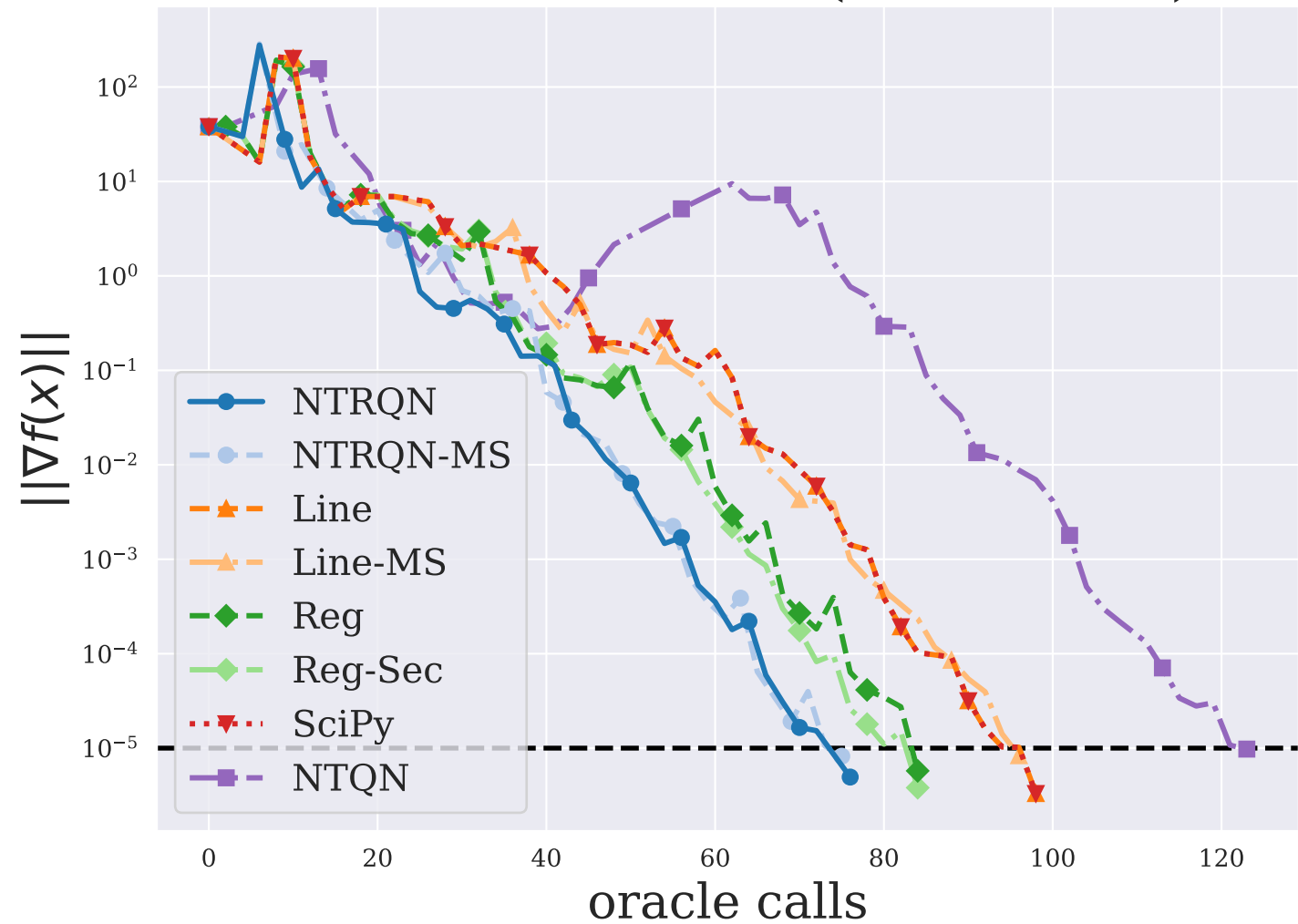
BROYDN3DLS ( n = 5000 )
