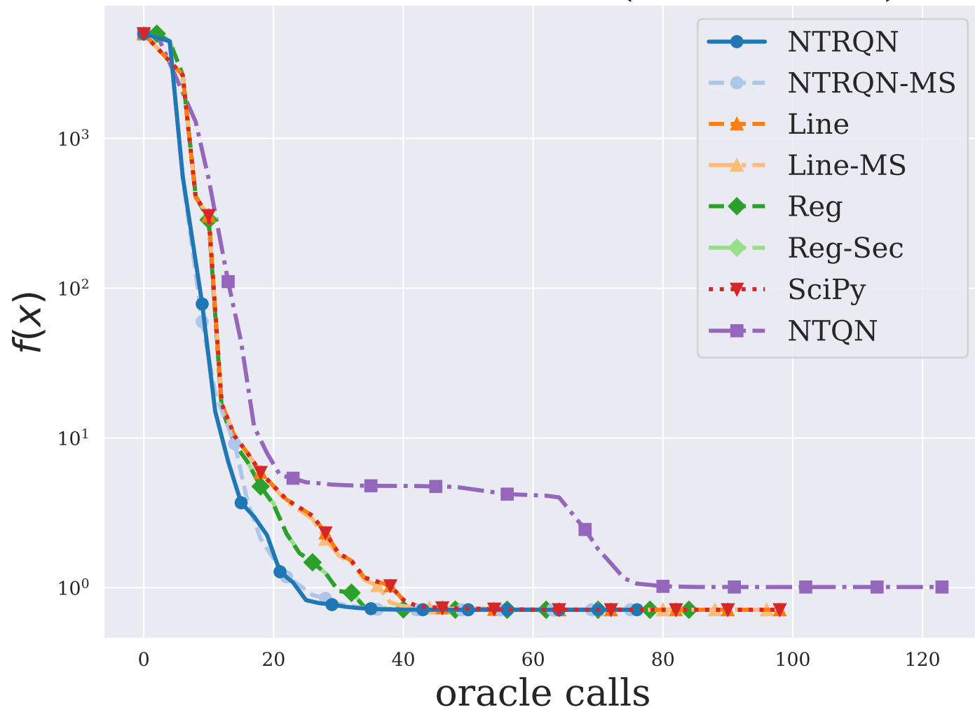
BROYDN3DLS ( n = 5000 )
