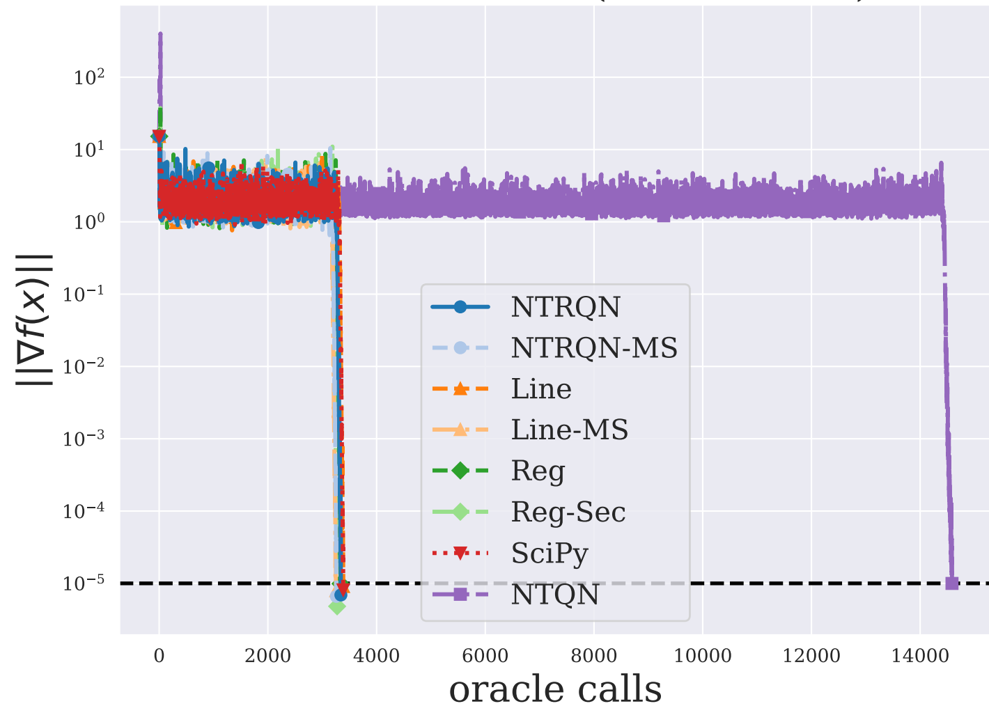
BROYDN7D ( n = 5000 )
