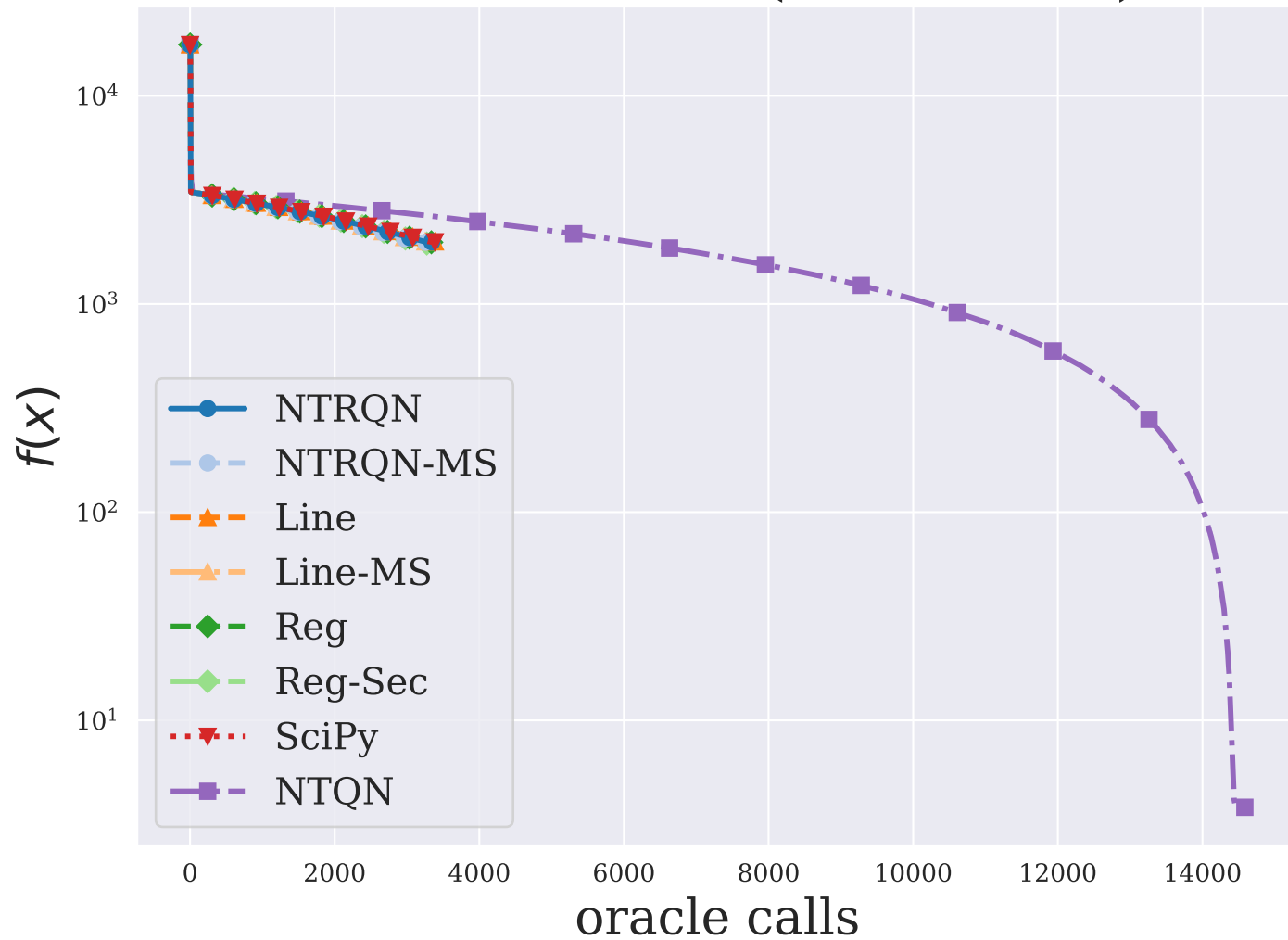
BROYDN7D ( n = 5000 )
