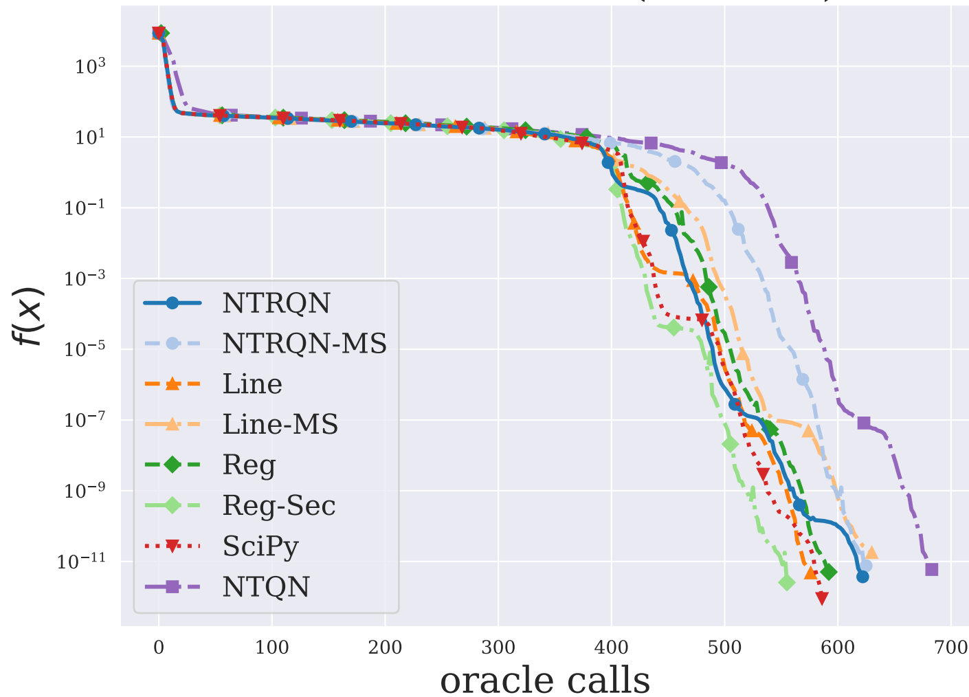
CHNRSNBM ( n = 50 )
