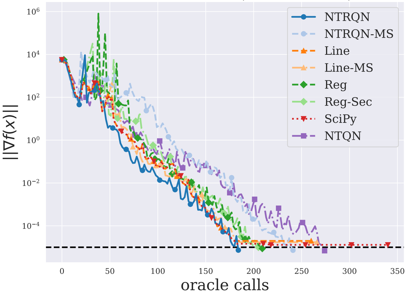
CRAGGLVY ( n = 5000 )
