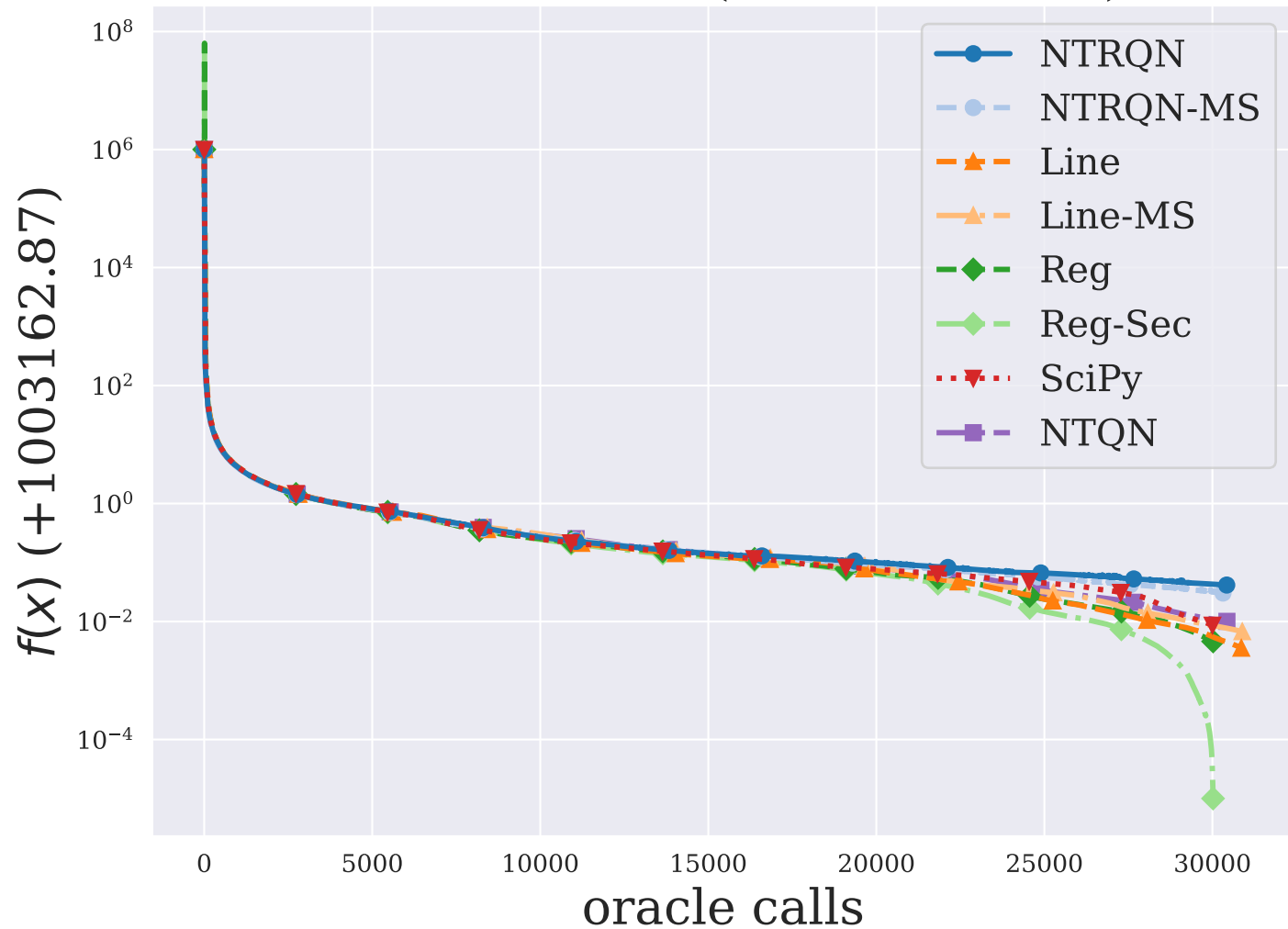
CURLY10 ( n = 10000 )
