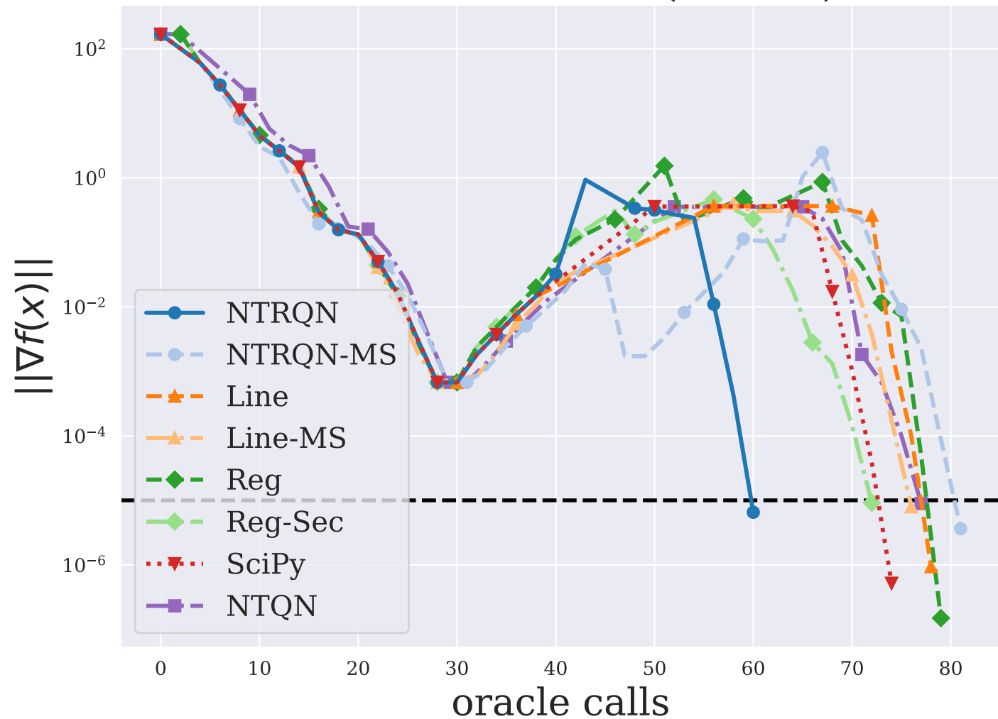
DENSCHNE ( n = 3 )
