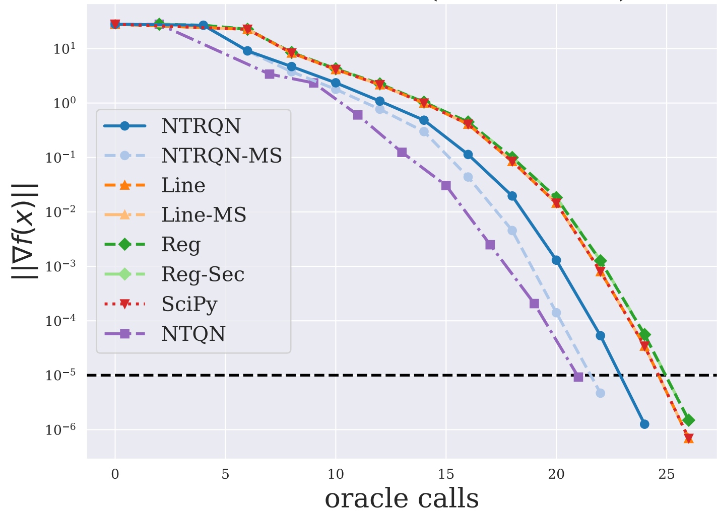
DIXMAANA ( n = 3000 )
