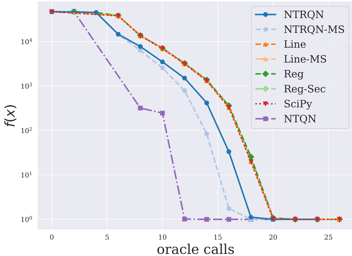
DIXMAANB ( n = 3000 )
