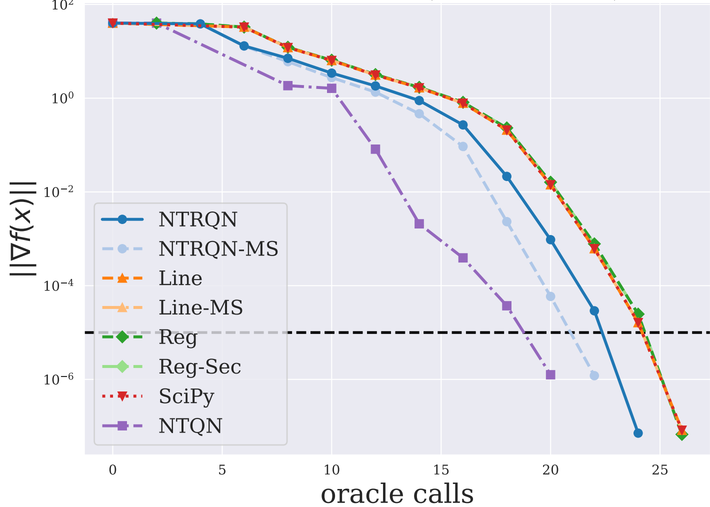
DIXMAANB ( n = 3000 )
