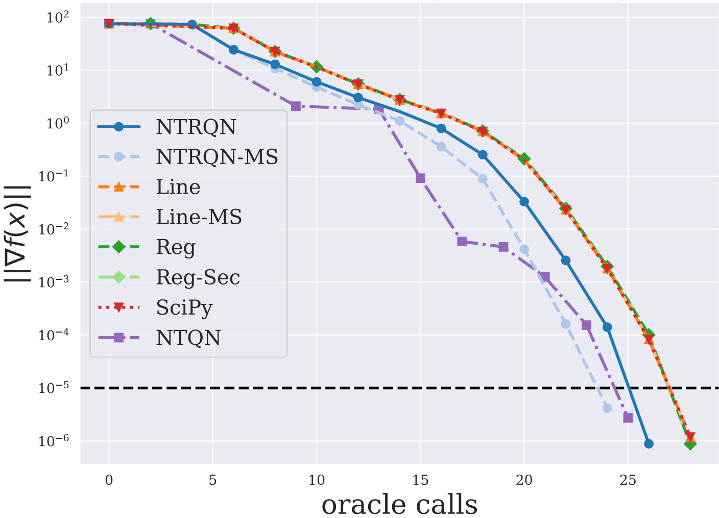
DIXMAANC ( n = 3000 )
