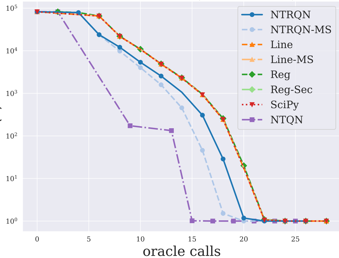
DIXMAANC ( n = 3000 )
