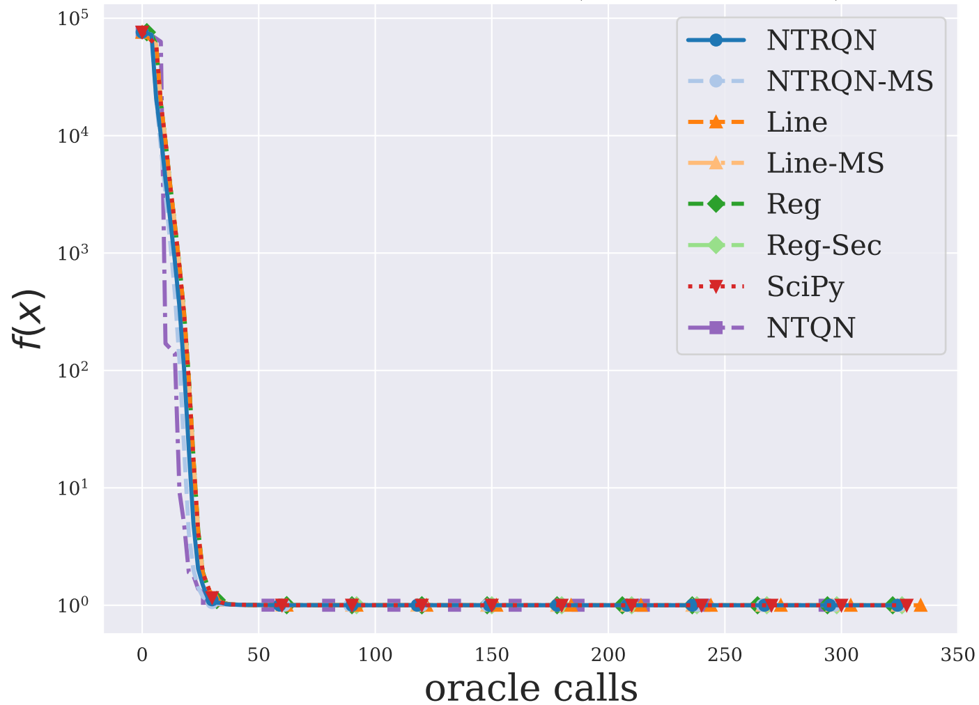
DIXMAANG ( n = 3000 )
