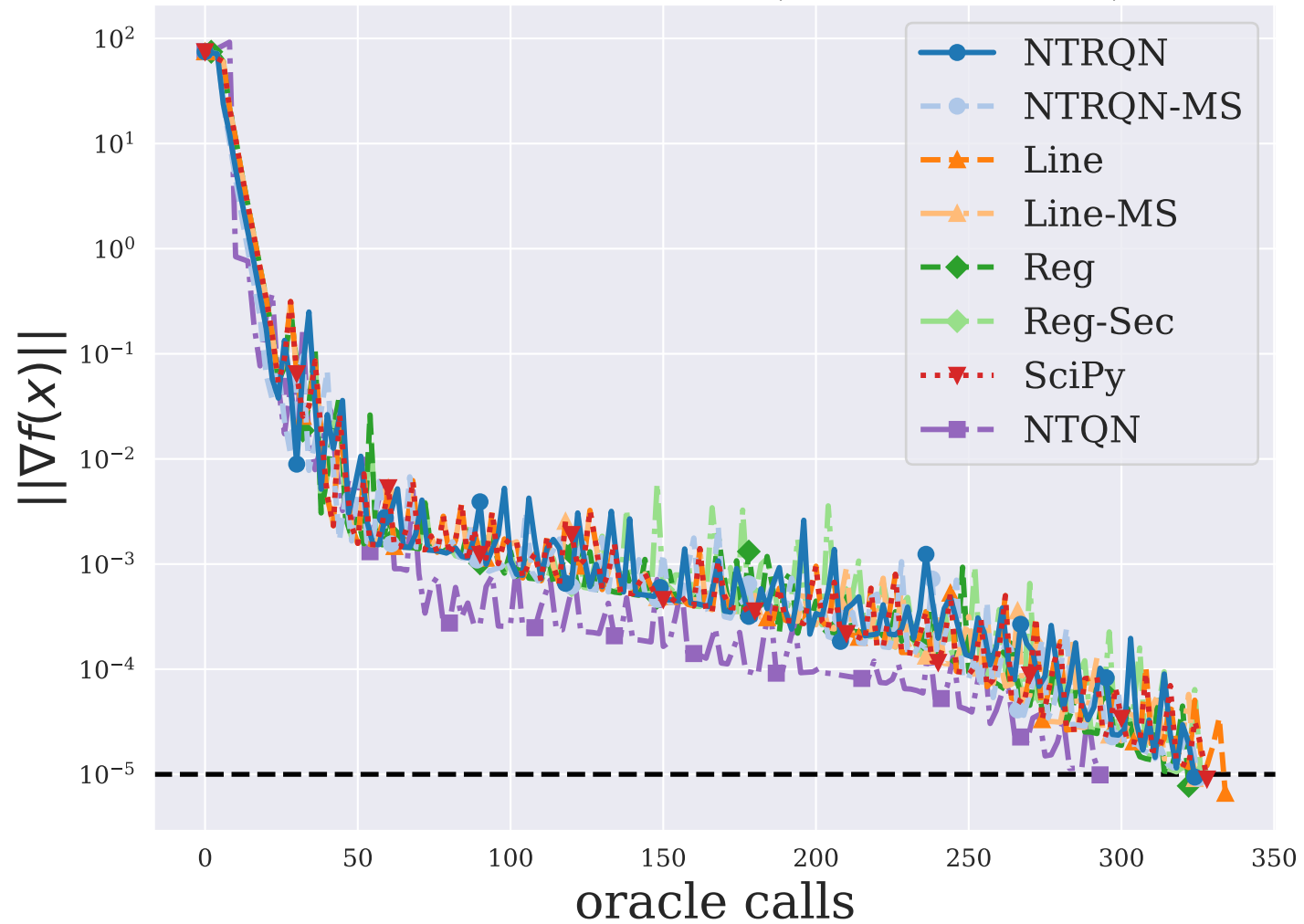
DIXMAANG ( n = 3000 )
