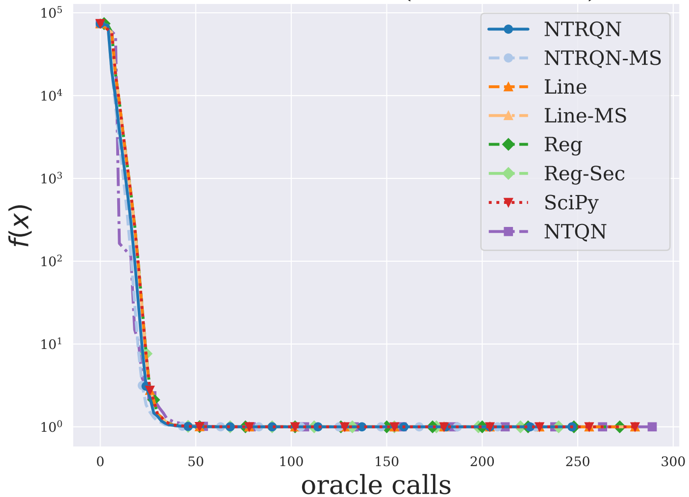
DIXMAANK ( n = 3000 )
