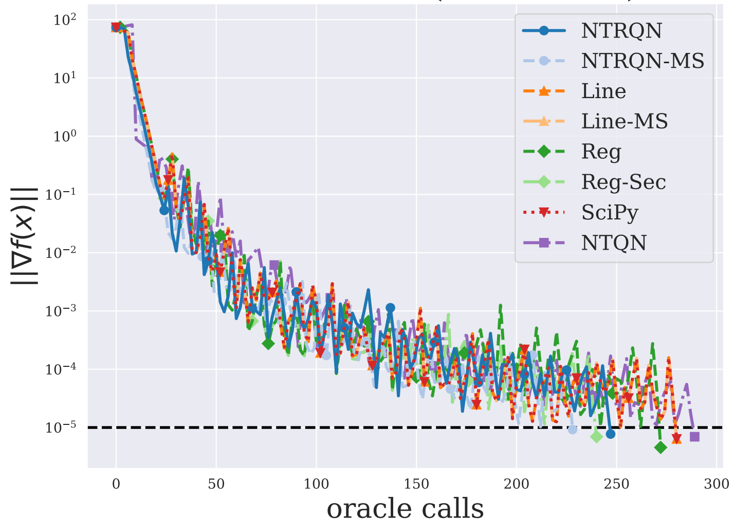
DIXMAANK ( n = 3000 )
