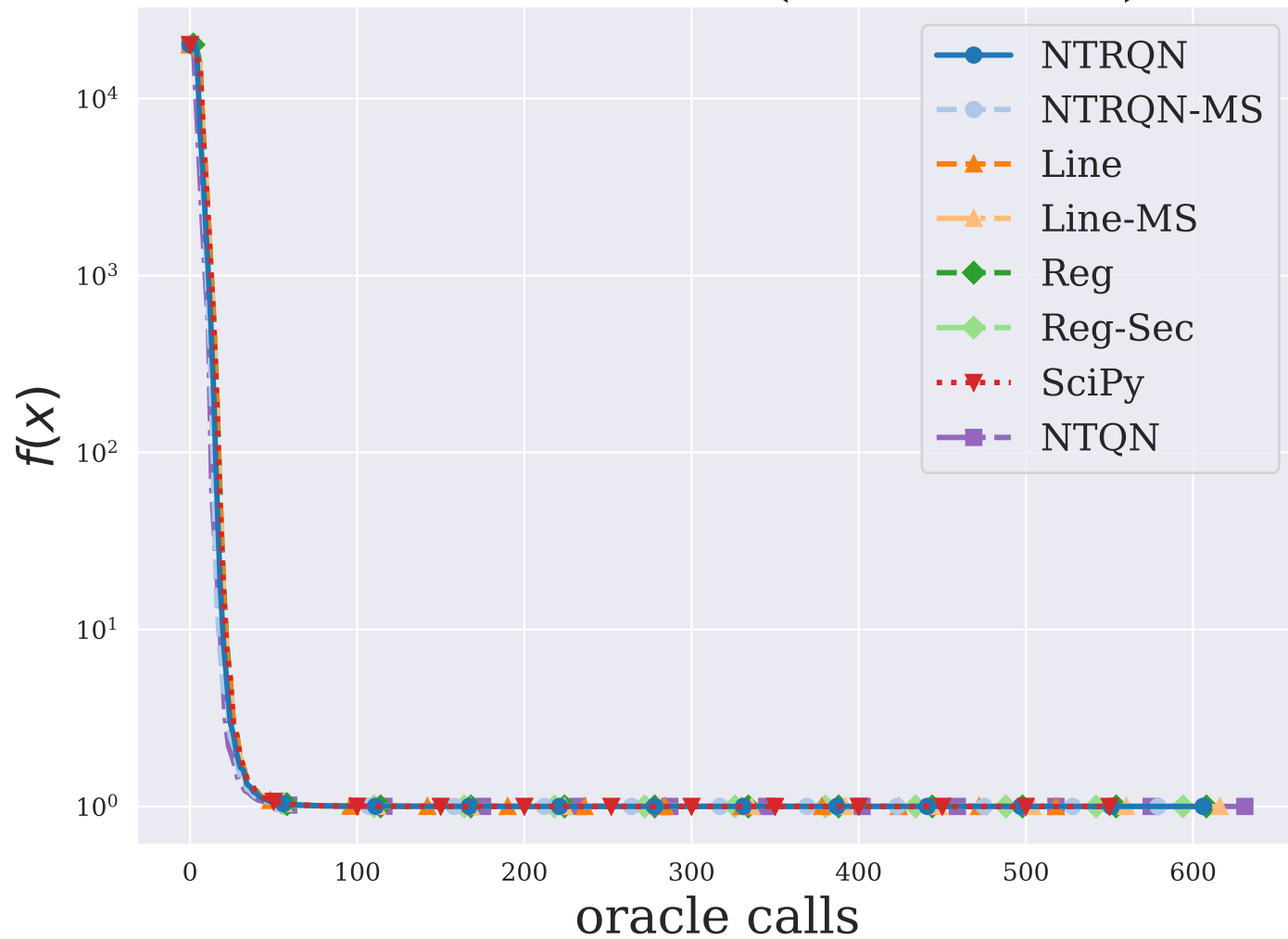
DIXMAANN ( n = 3000 )
