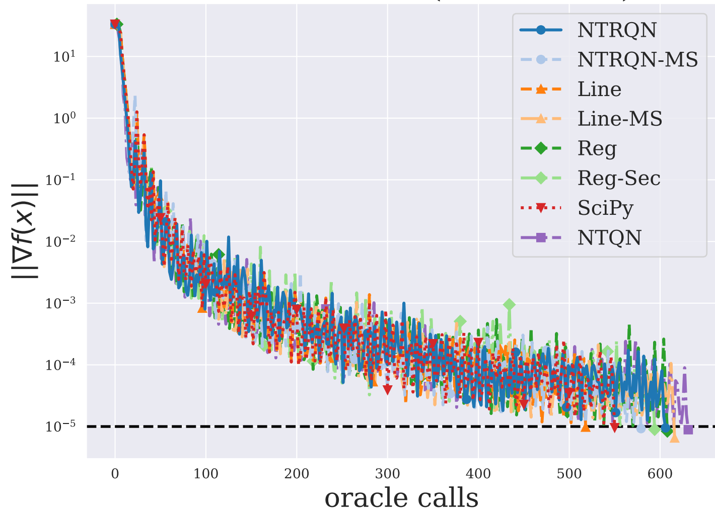
DIXMAANN ( n = 3000 )
