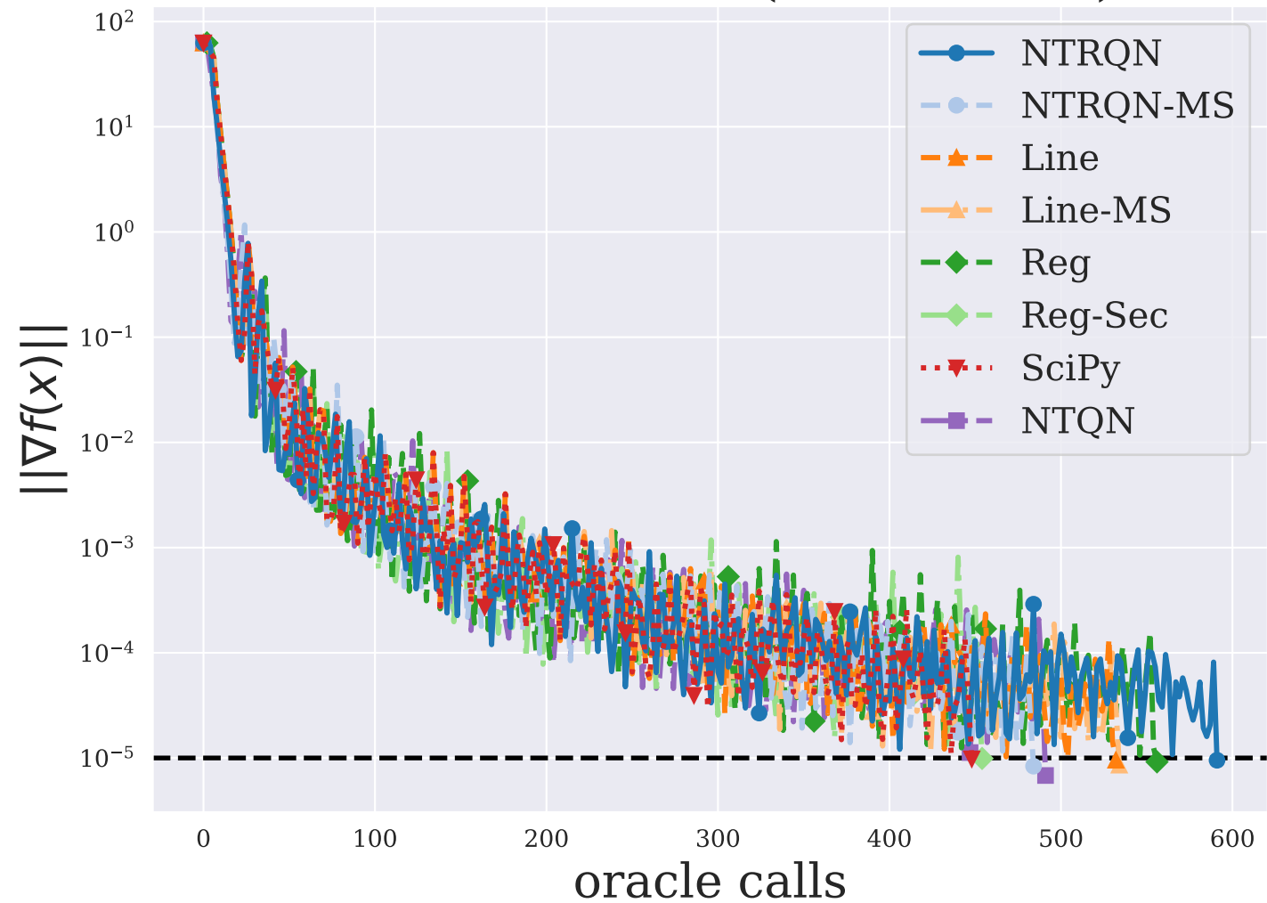
DIXMAANO ( n = 3000 )
