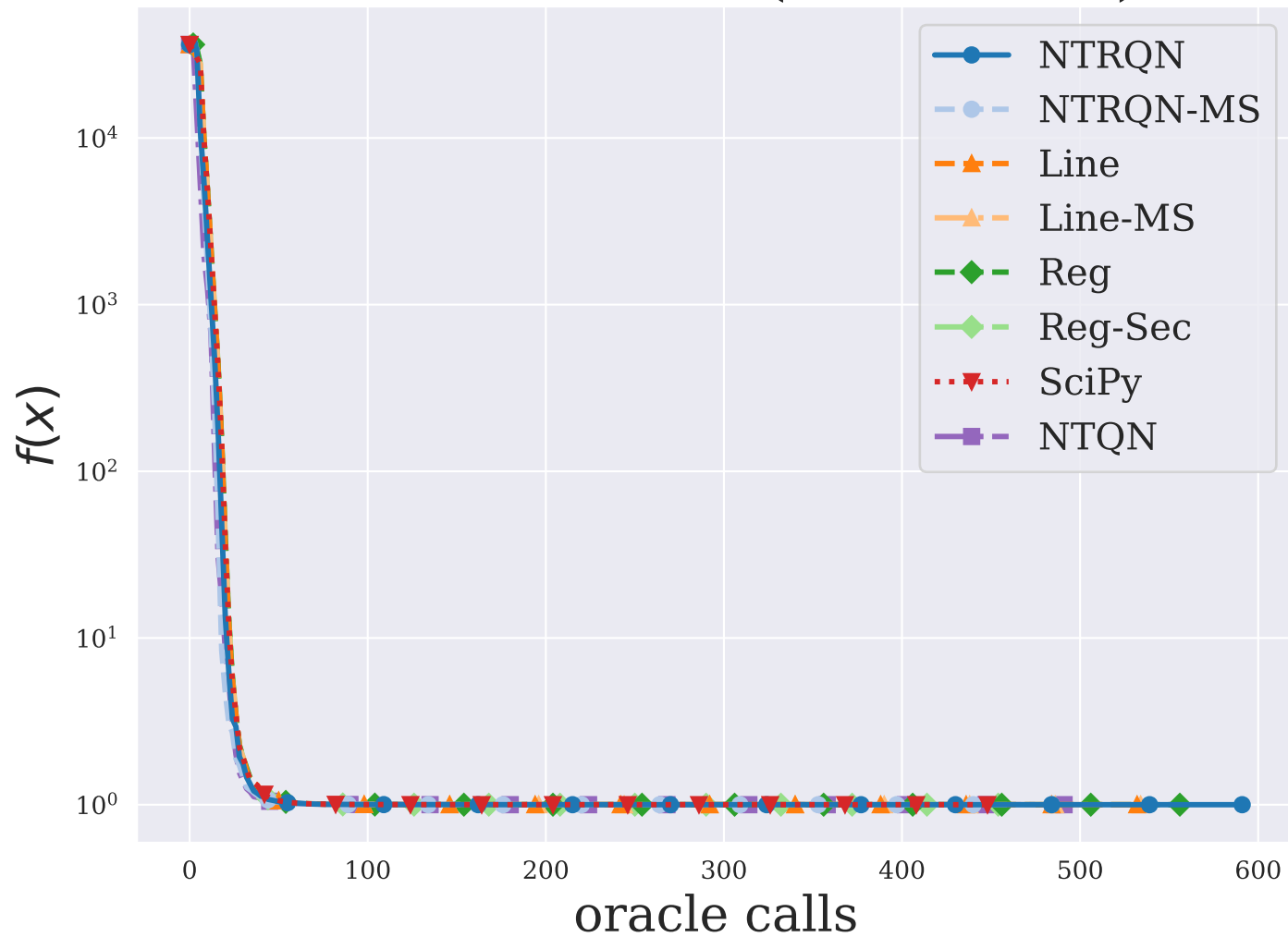
DIXMAANO ( n = 3000 )
