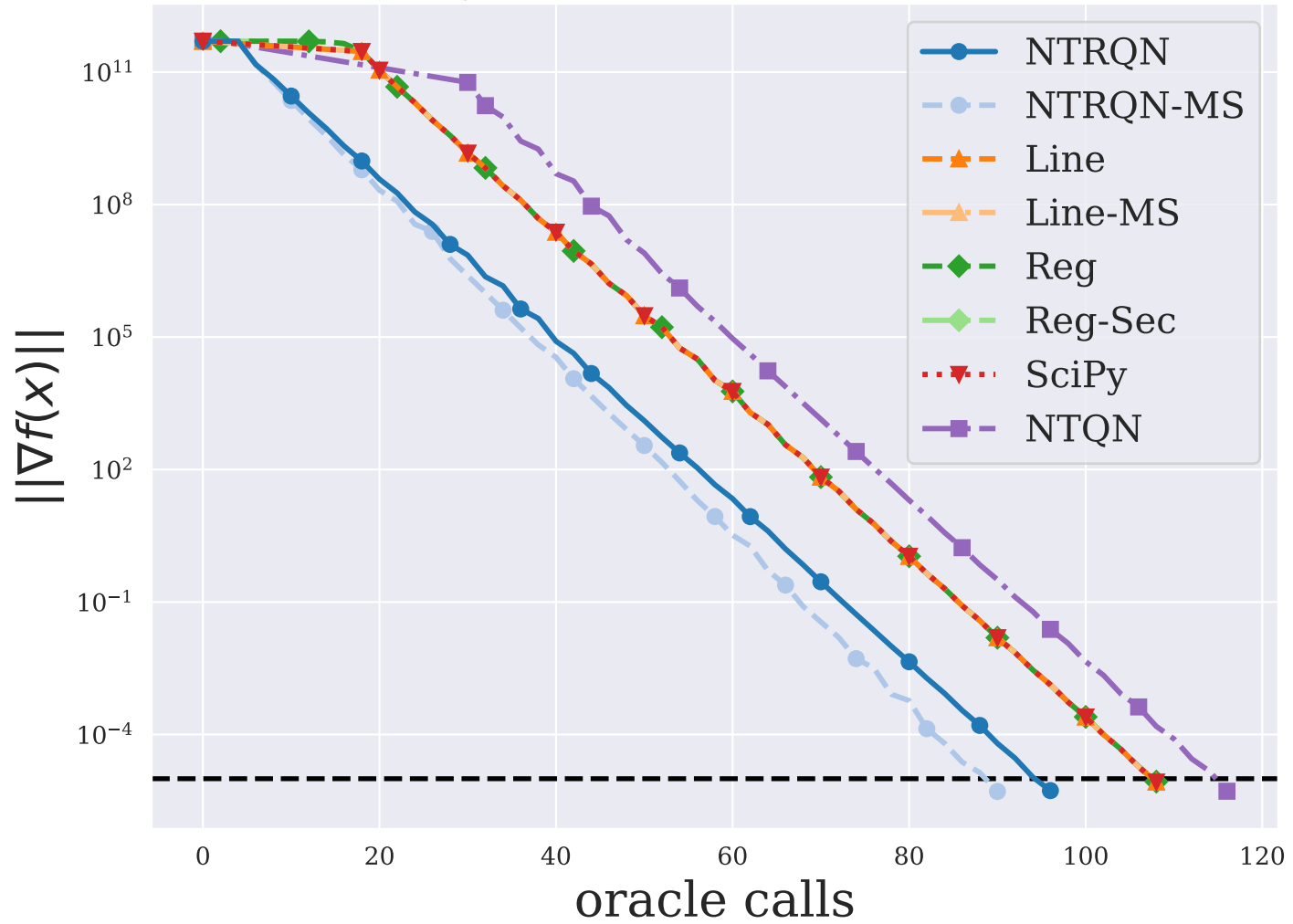
DQRTIC ( n = 5000 )
