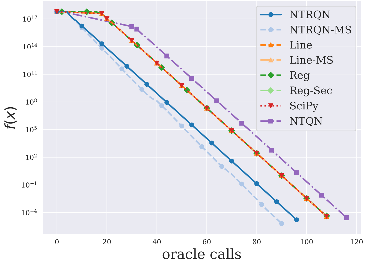
DQRTIC ( n = 5000 )
