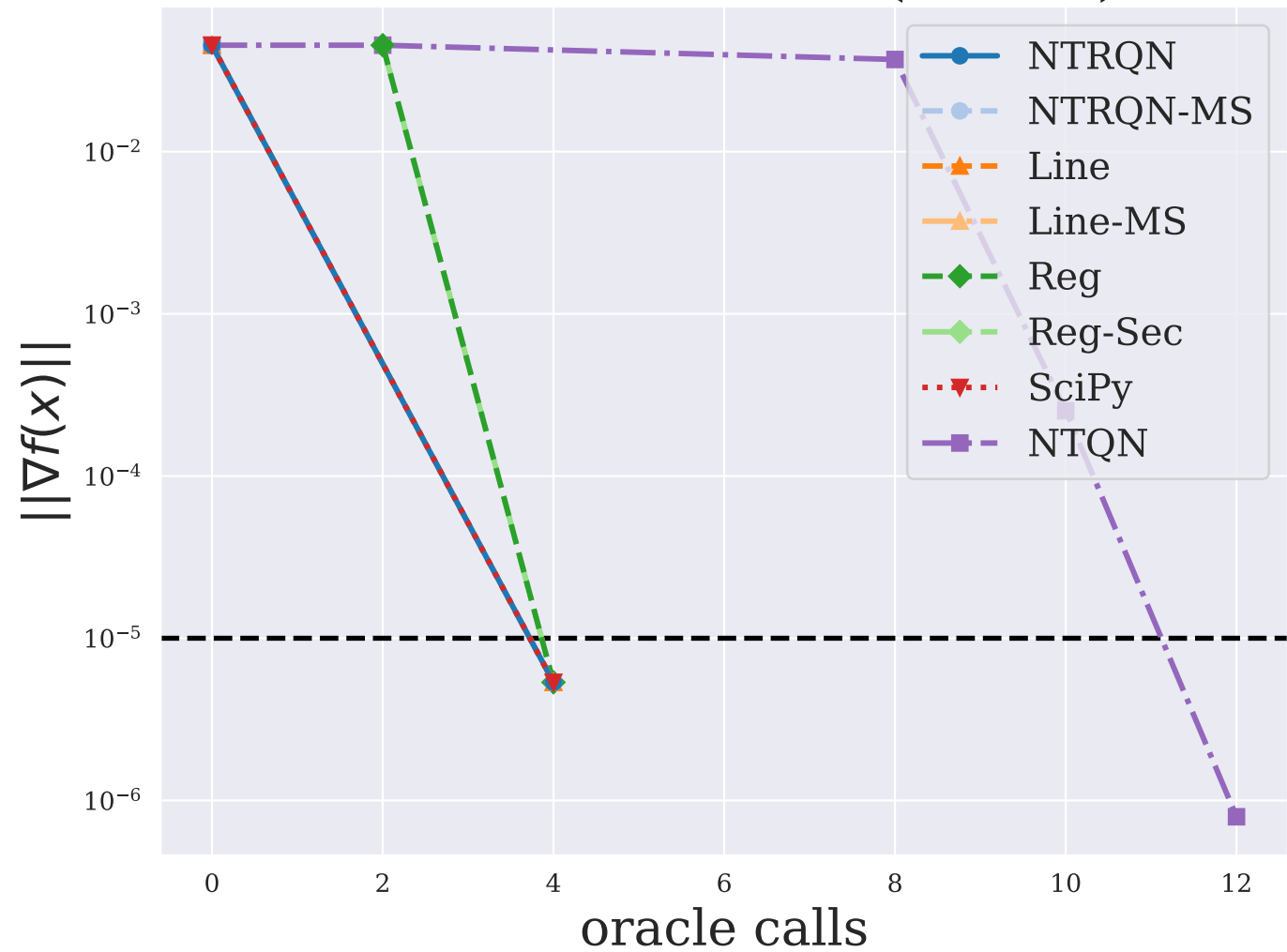
ECKERLE4LS ( n = 3 )
