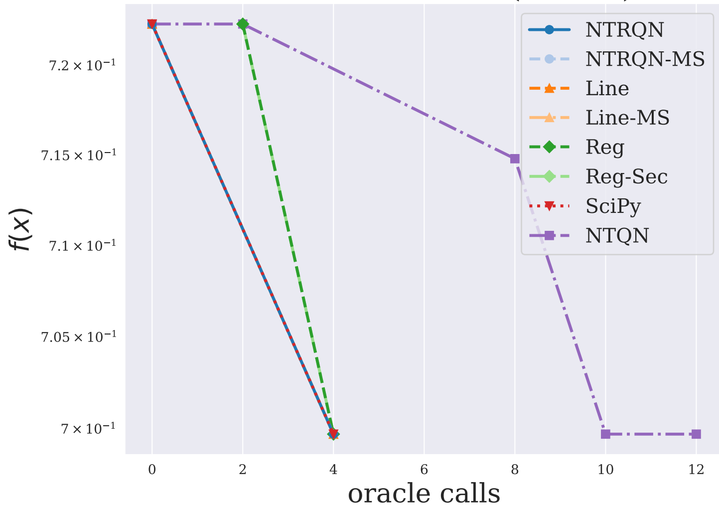
ECKERLE4LS ( n = 3 )
