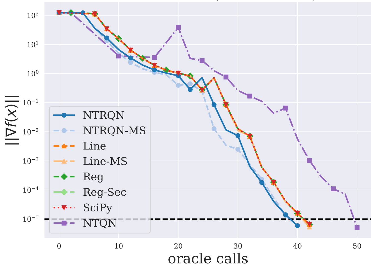
ENGVAL1 ( n = 5000 )
