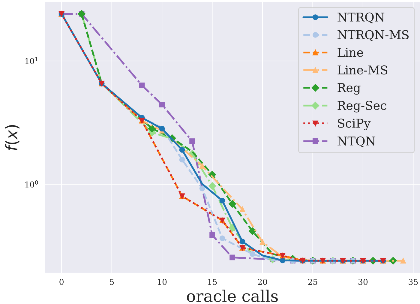
EXPFIT ( n = 2 )
