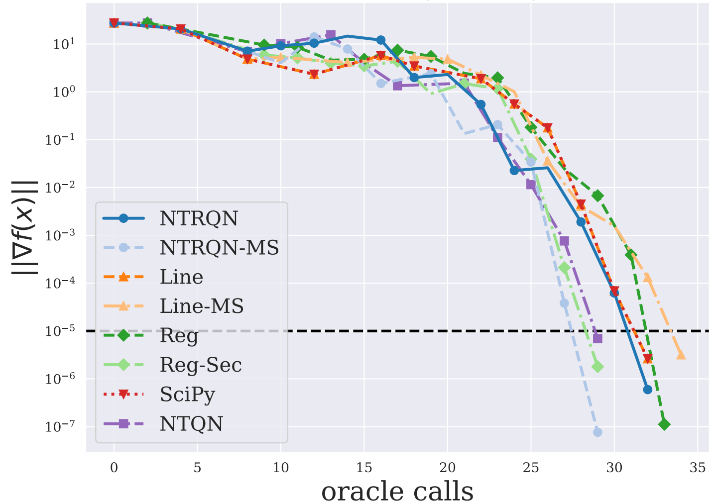
EXPFIT ( n = 2 )
