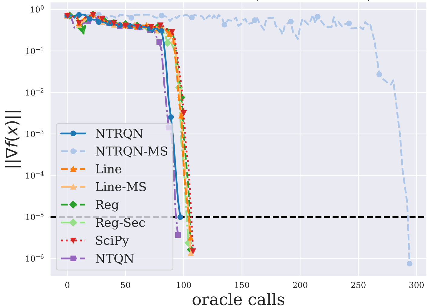
FLETBV3M ( n = 5000 )
