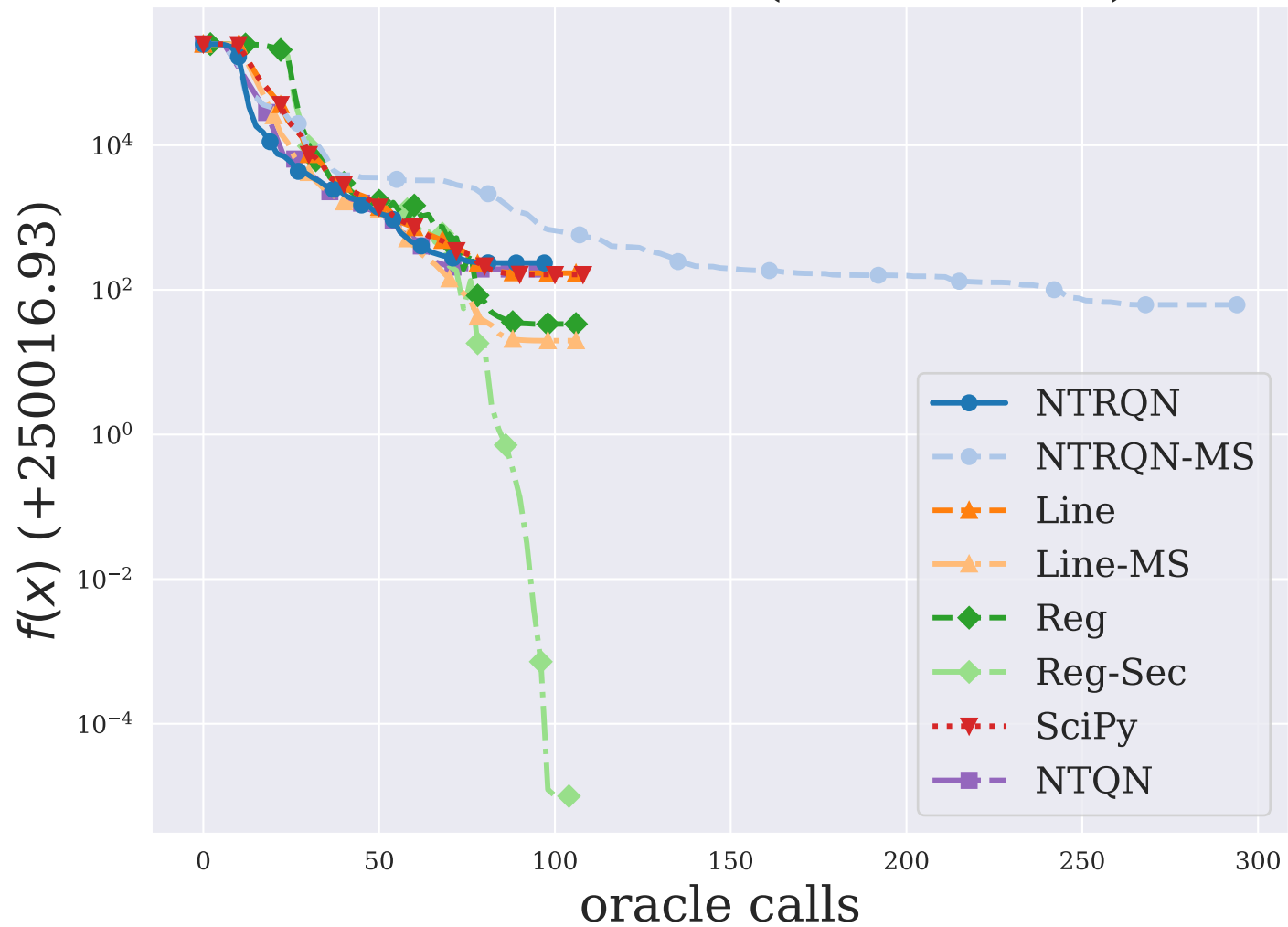
FLETBV3M ( n = 5000 )
