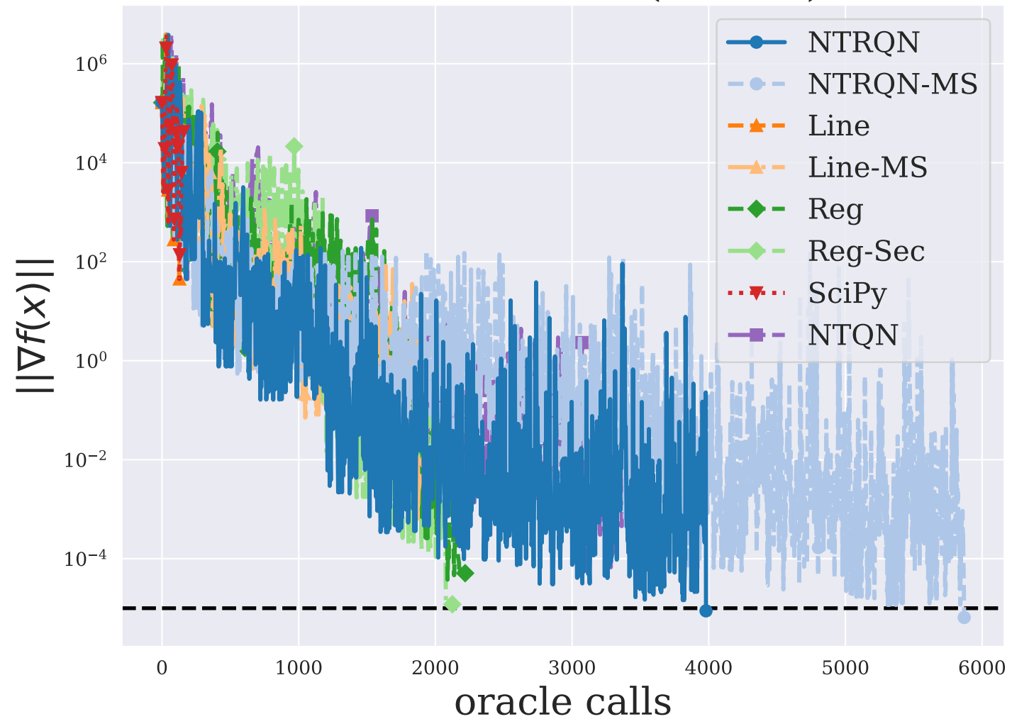
GAUSS1LS ( n = 8 )
