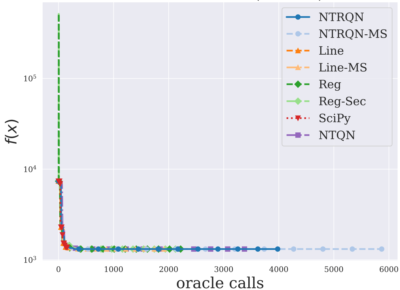
GAUSS1LS ( n = 8 )
