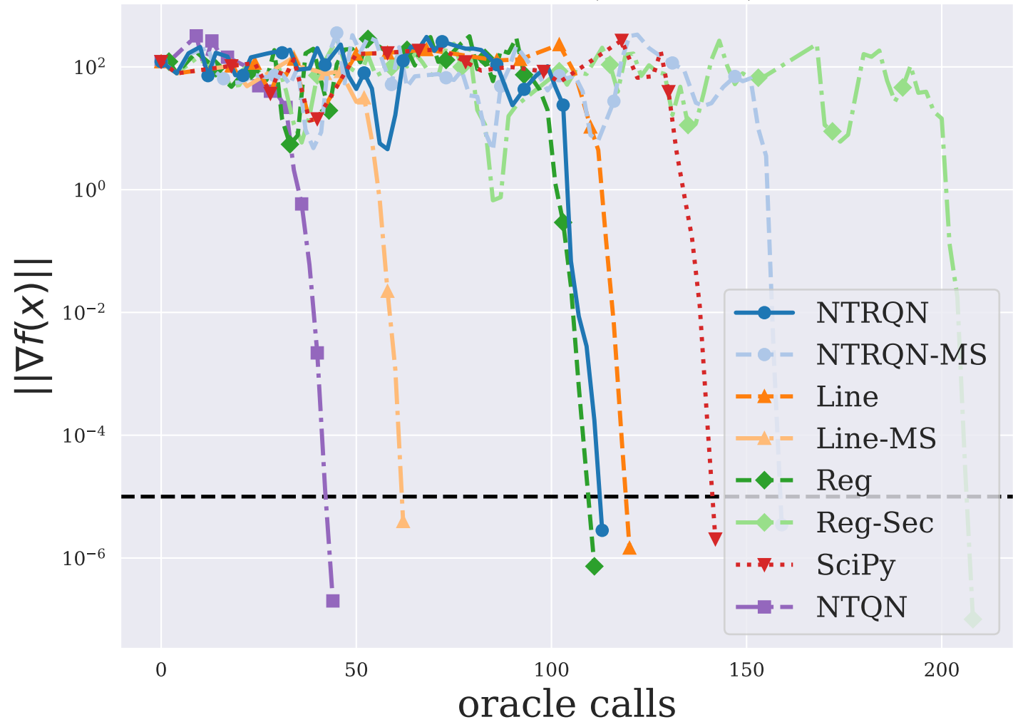
HAIRY ( n = 2 )
