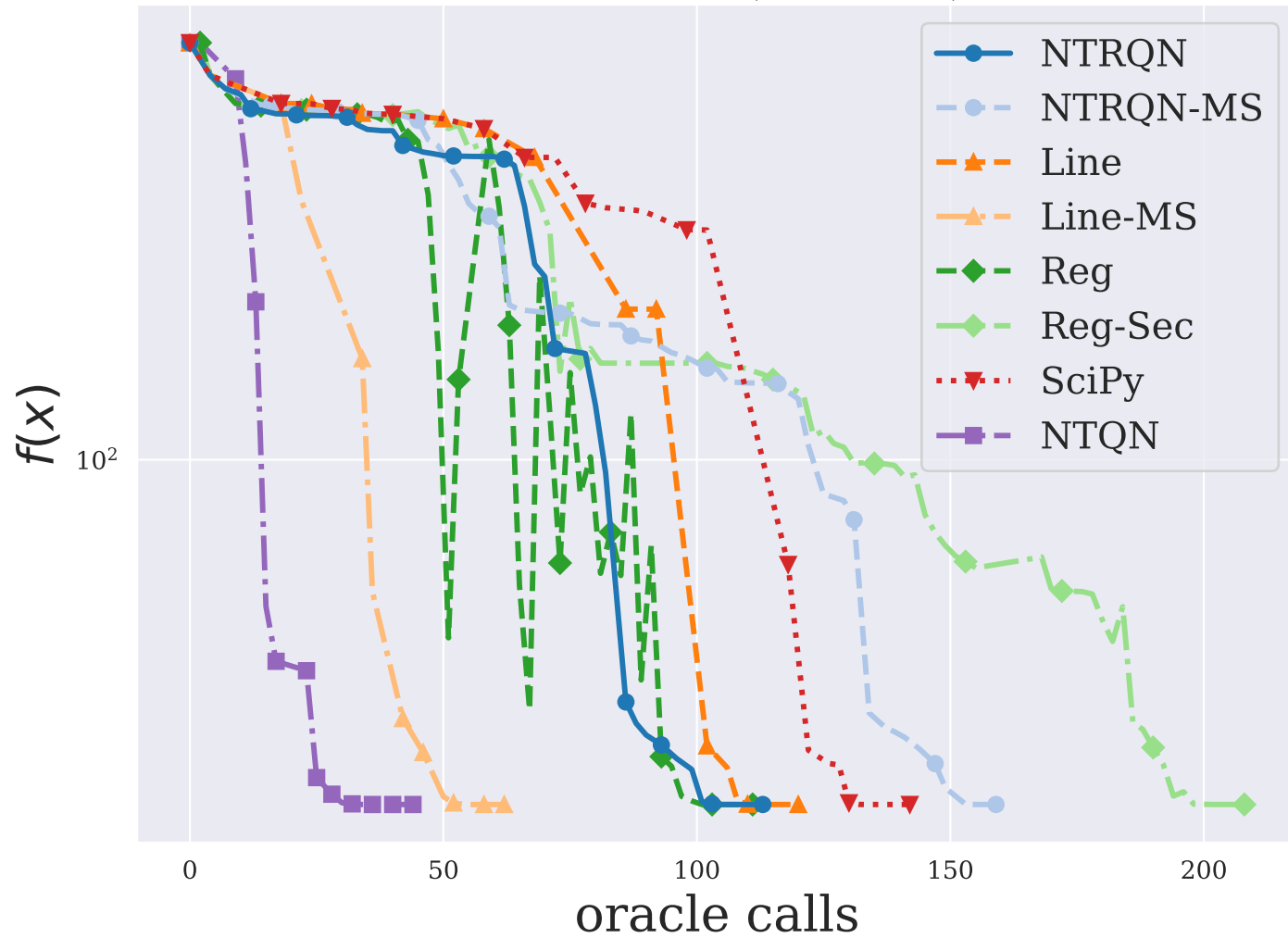
HAIRY ( n = 2 )
