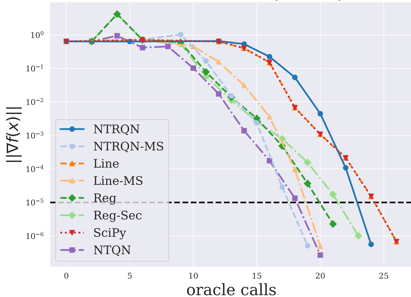
HIMMELBG ( n = 2 )
