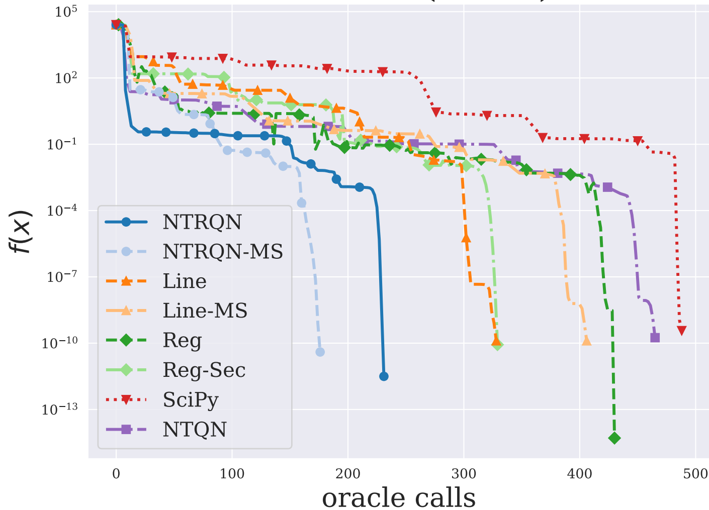
HUMPS ( n = 2 )
