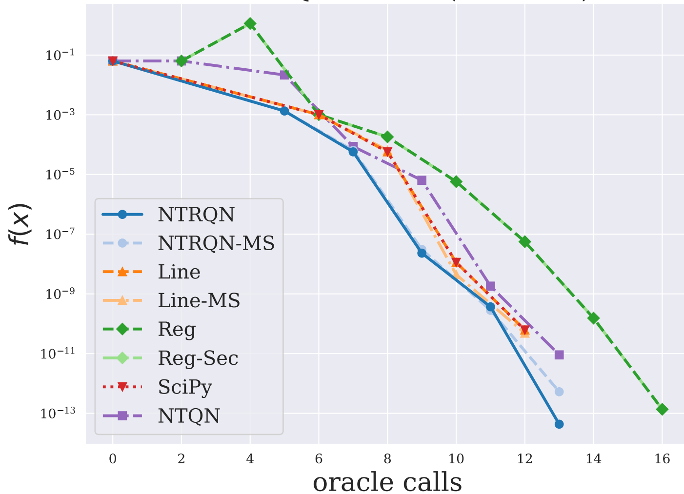
INTEQNELS ( n = 12 )
