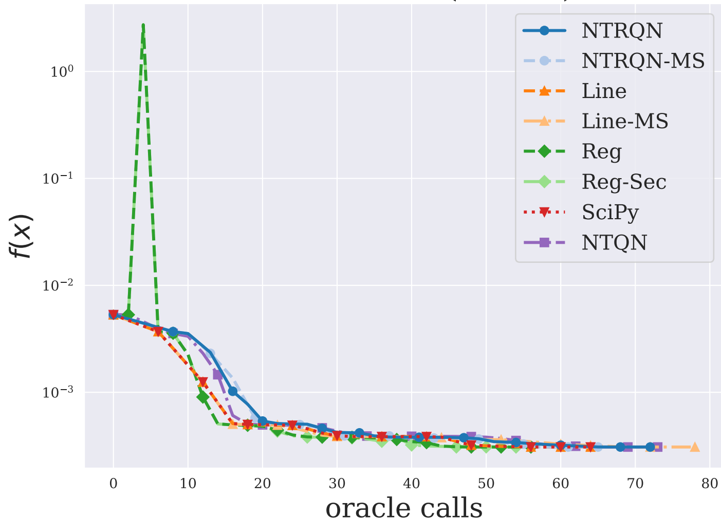
KOWOSB ( n = 4 )
