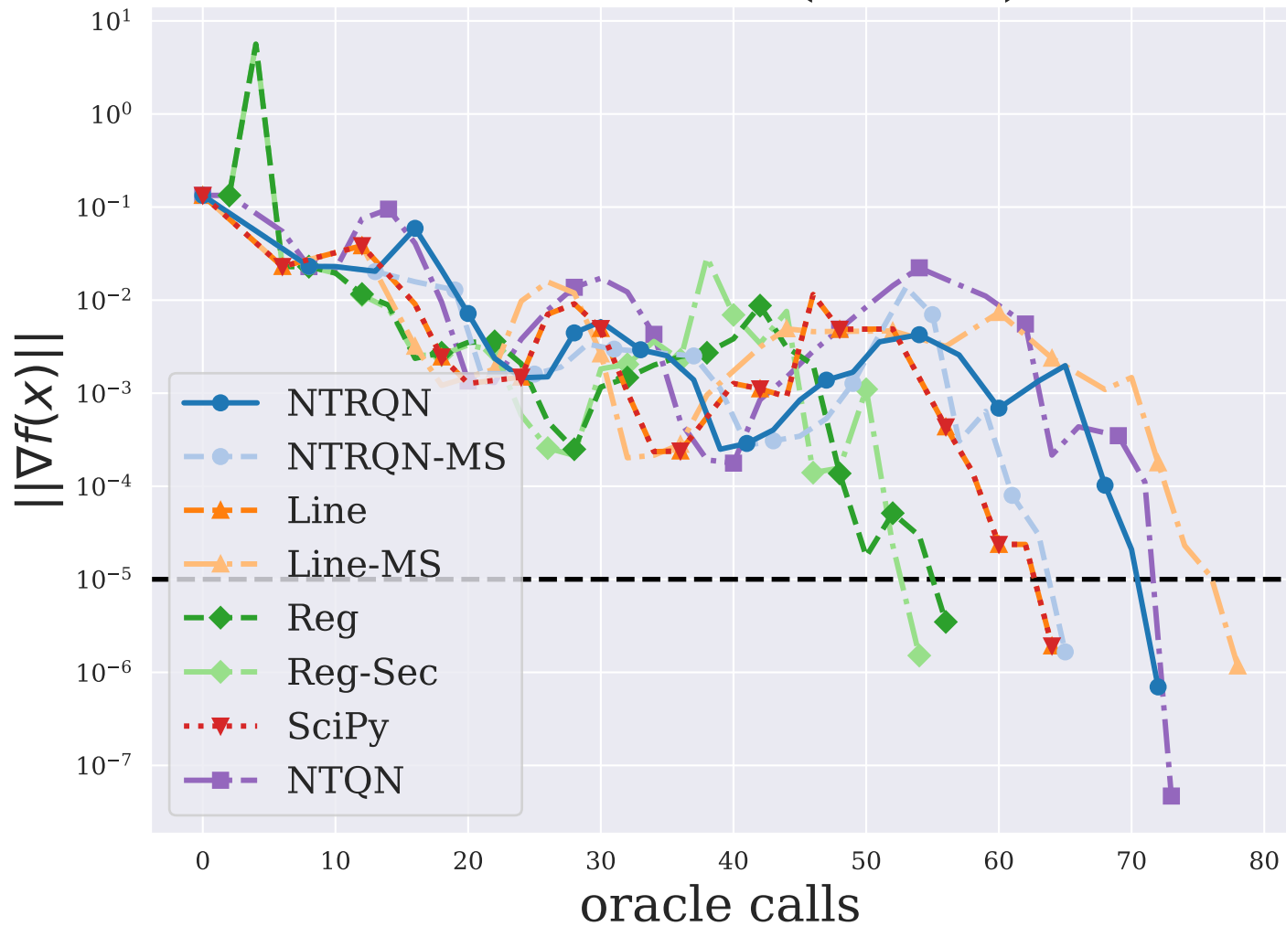
KOWOSB ( n = 4 )
