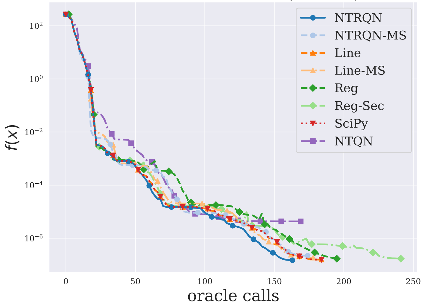
LANCZOS1LS ( n = 6 )
