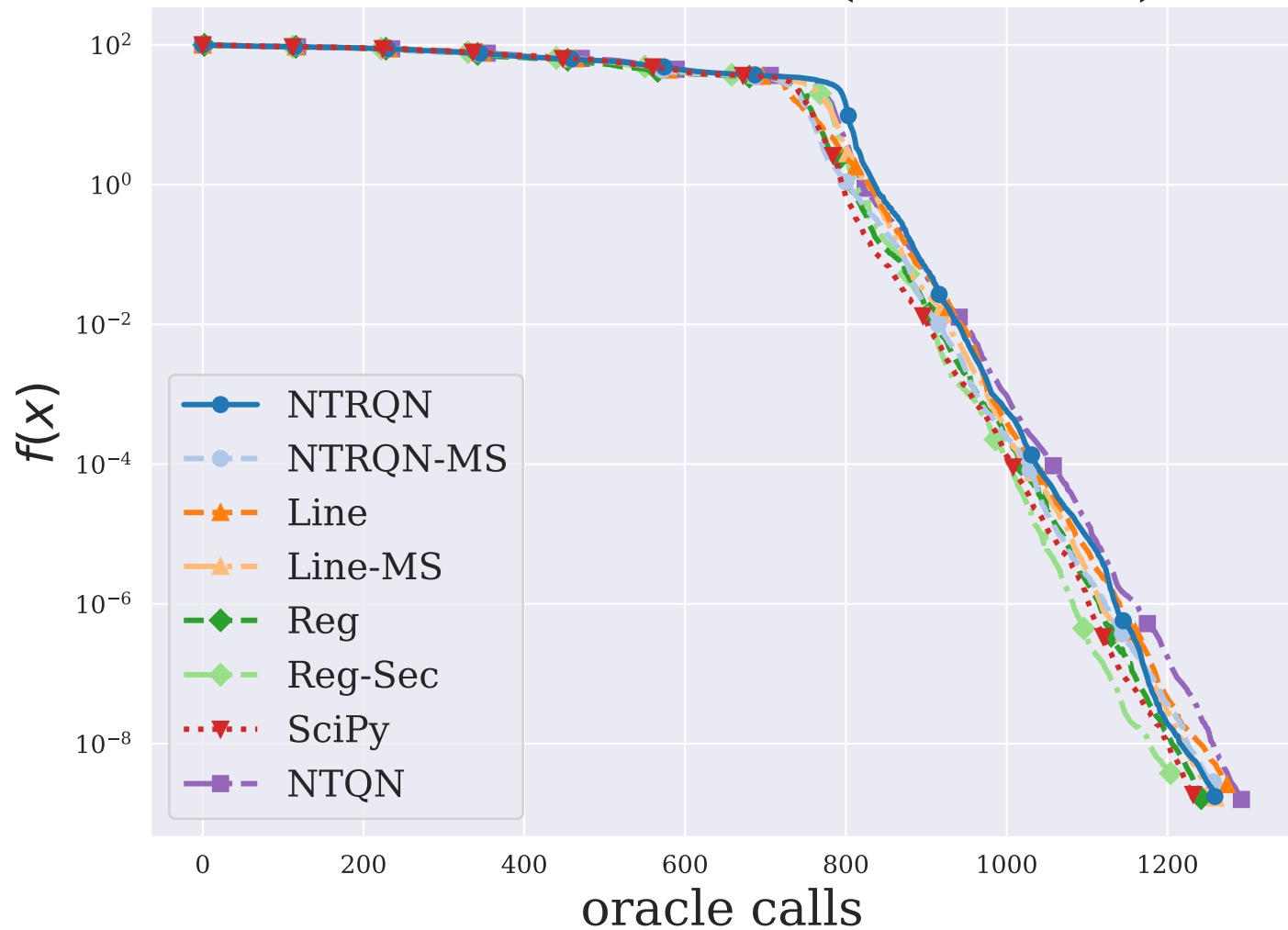
LUKSAN21LS ( n = 100 )
