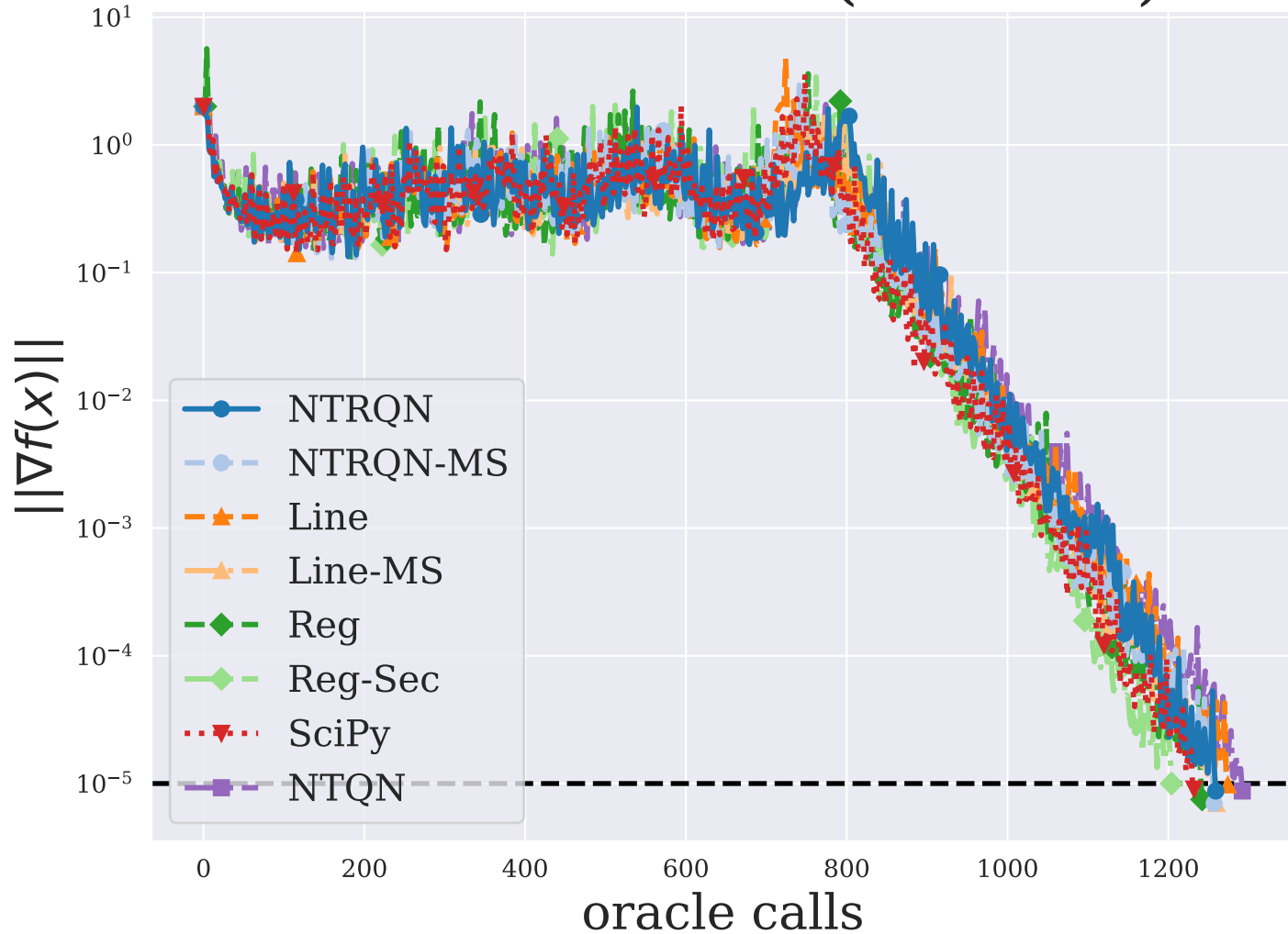
LUKSAN21LS ( n = 100 )
