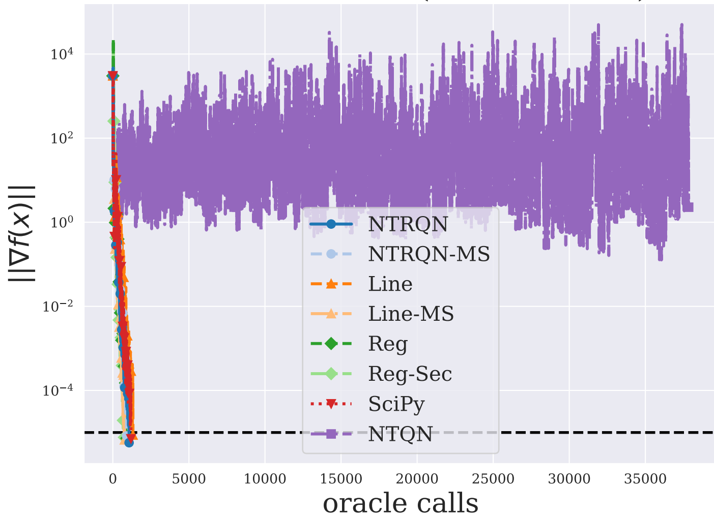
MODBEALE ( n = 20000 )
