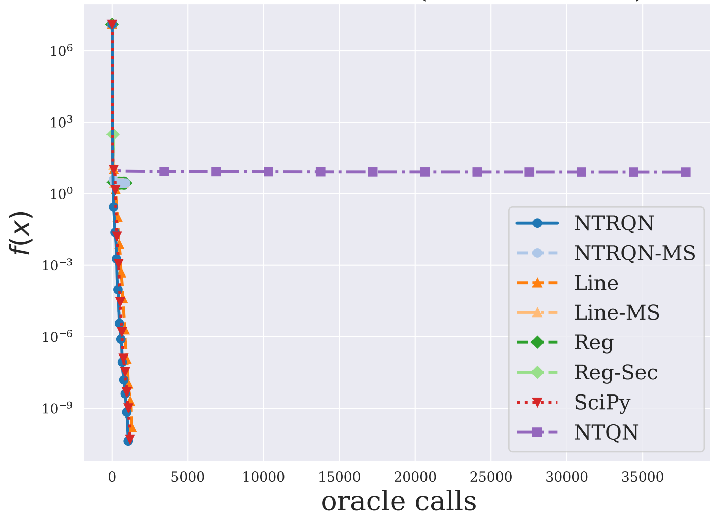
MODBEALE ( n = 20000 )
