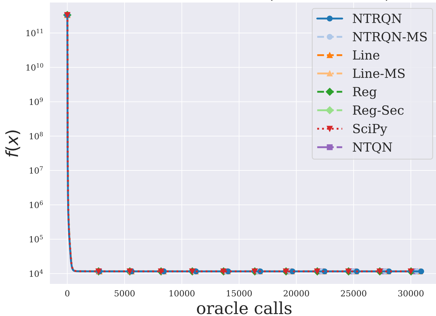
NONCVXUN ( n = 5000 )
