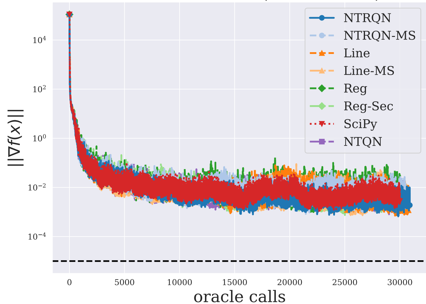
NONCVXUN ( n = 5000 )
