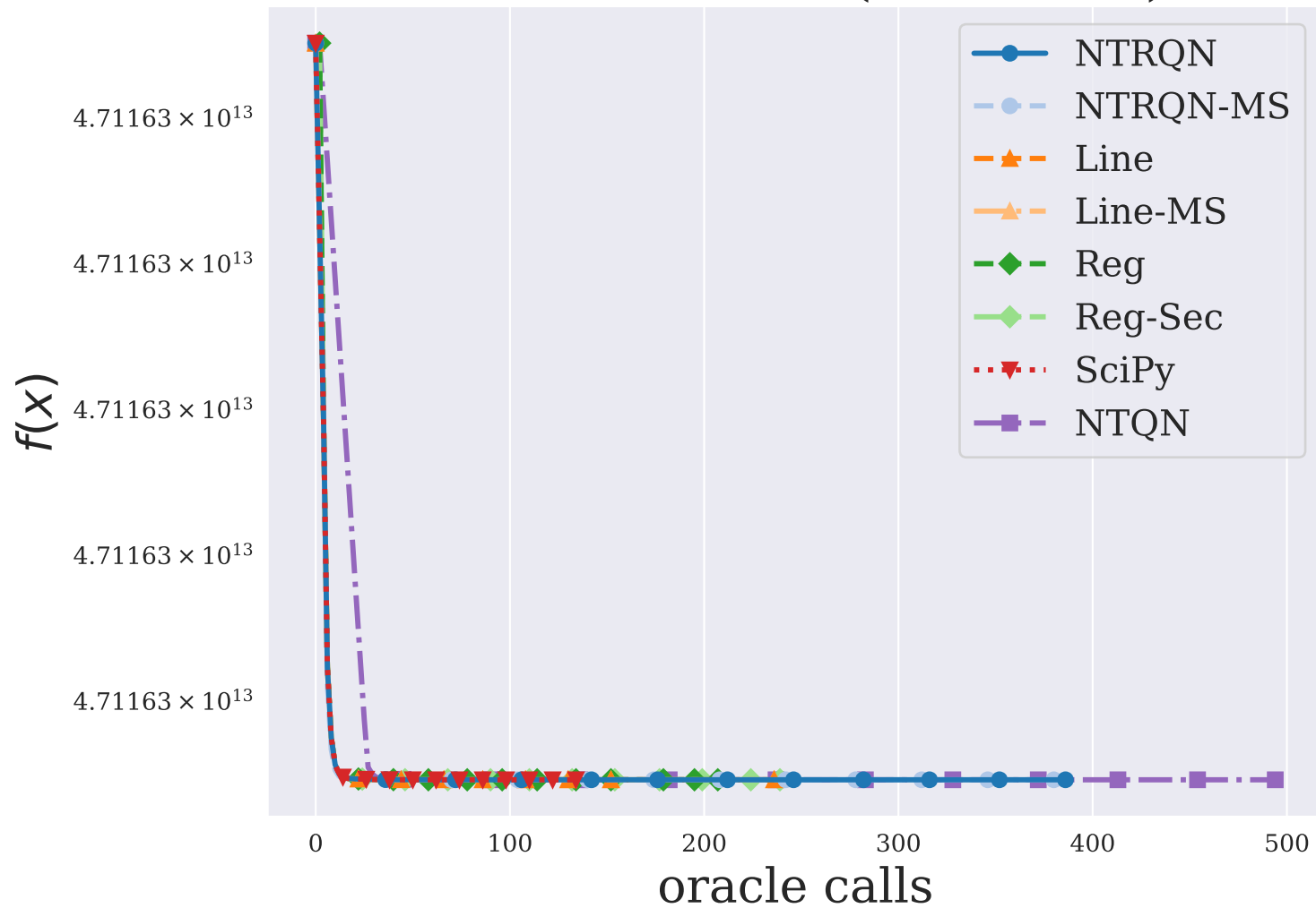
PENALTY2 ( n = 200 )
