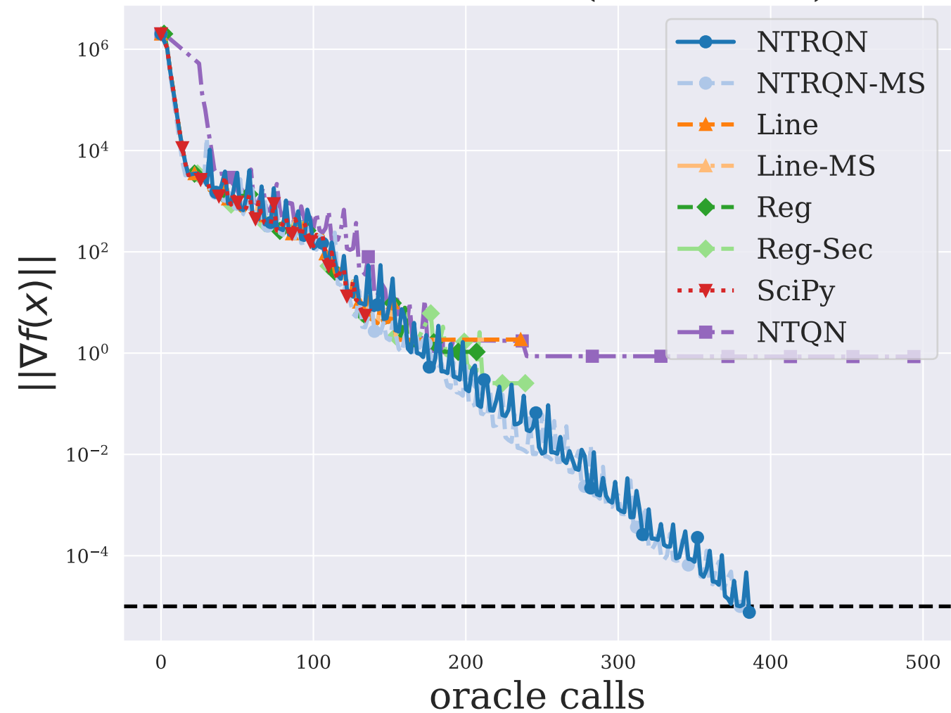
PENALTY2 ( n = 200 )
