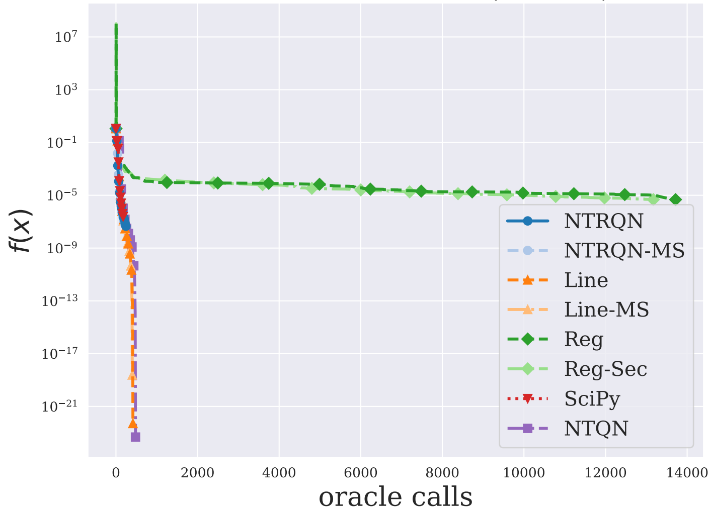
POWELLBSLS ( n = 2 )
