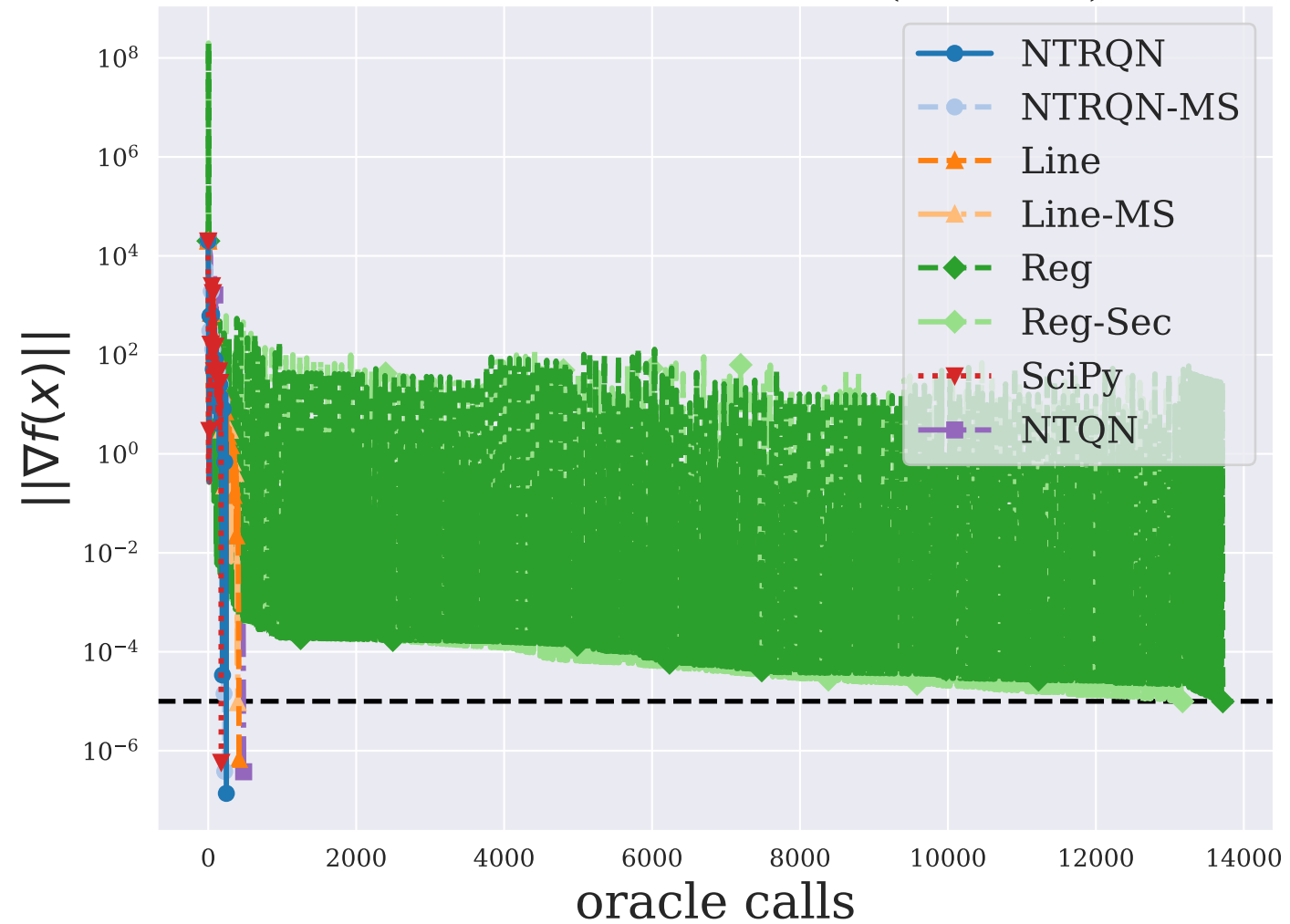
POWELLBSLS ( n = 2 )
