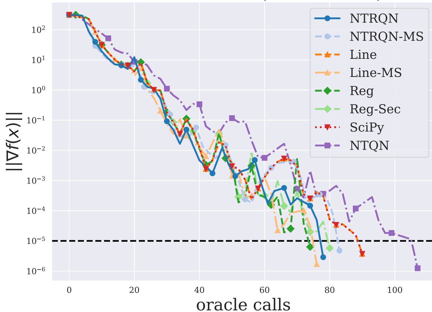
POWELLSG ( n = 5000 )
