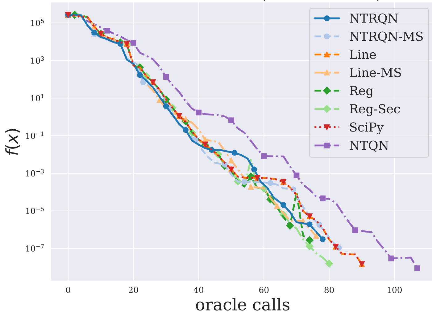
POWELLSG ( n = 5000 )
