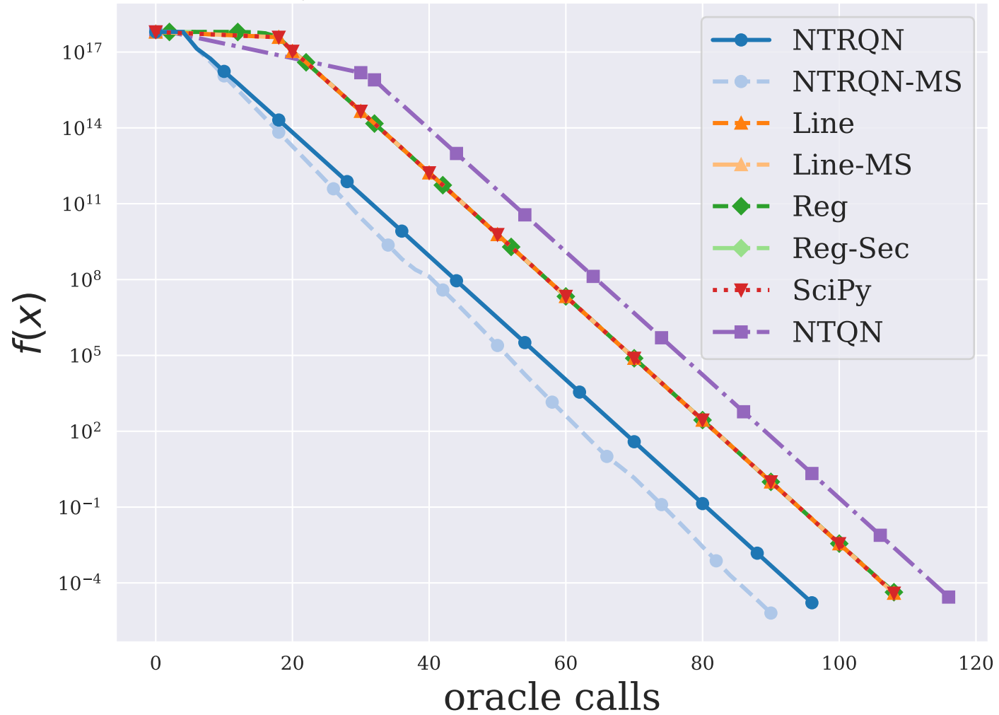
QUARTC ( n = 5000 )
