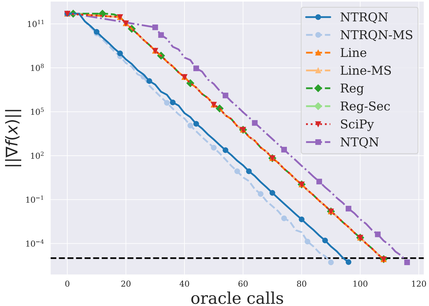
QUARTC ( n = 5000 )
