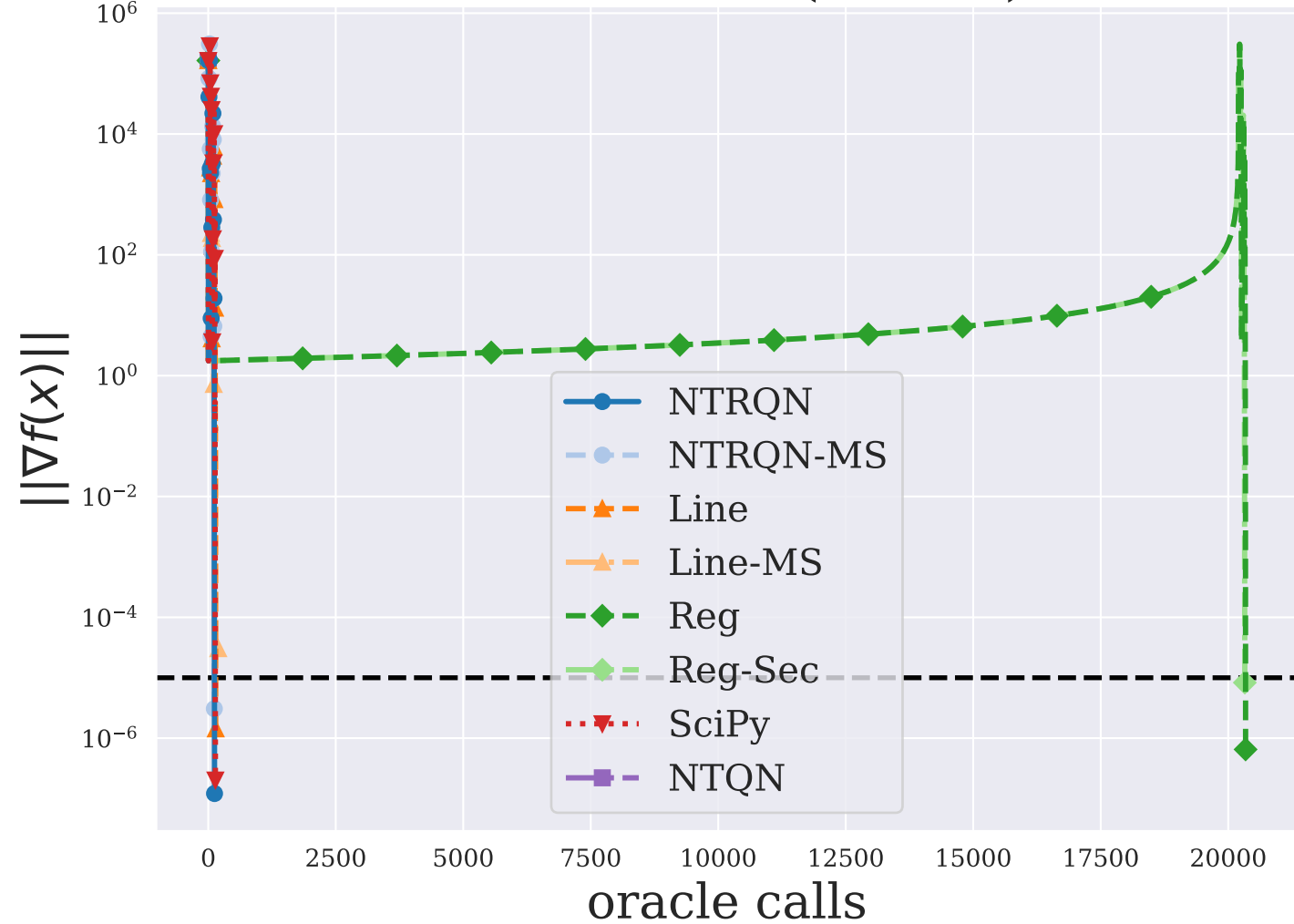
RAT42LS ( n = 3 )
