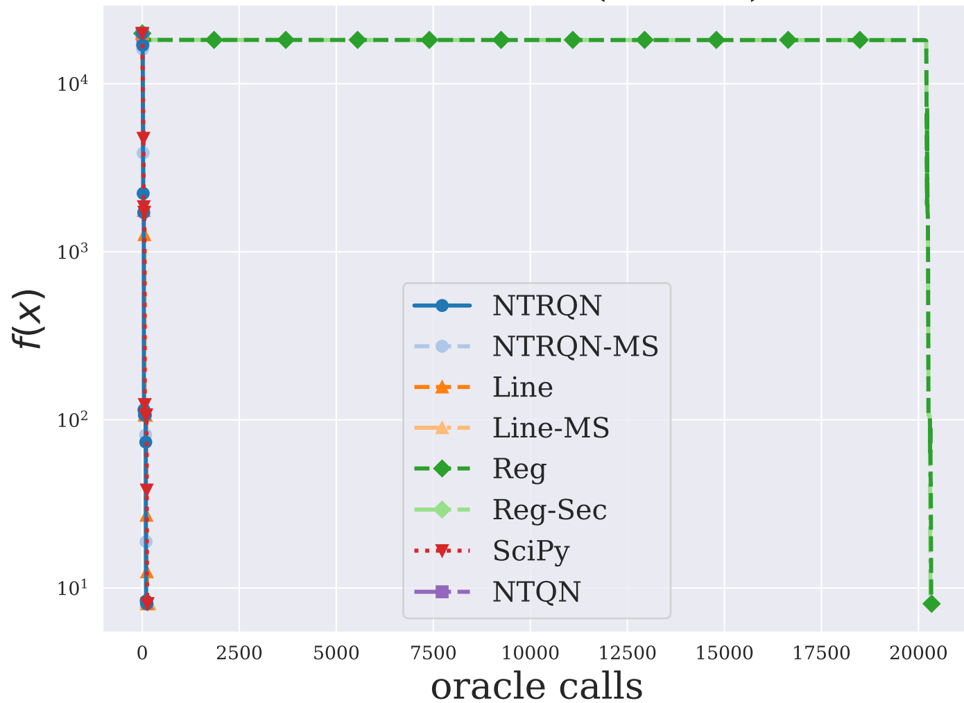
RAT42LS ( n = 3 )
