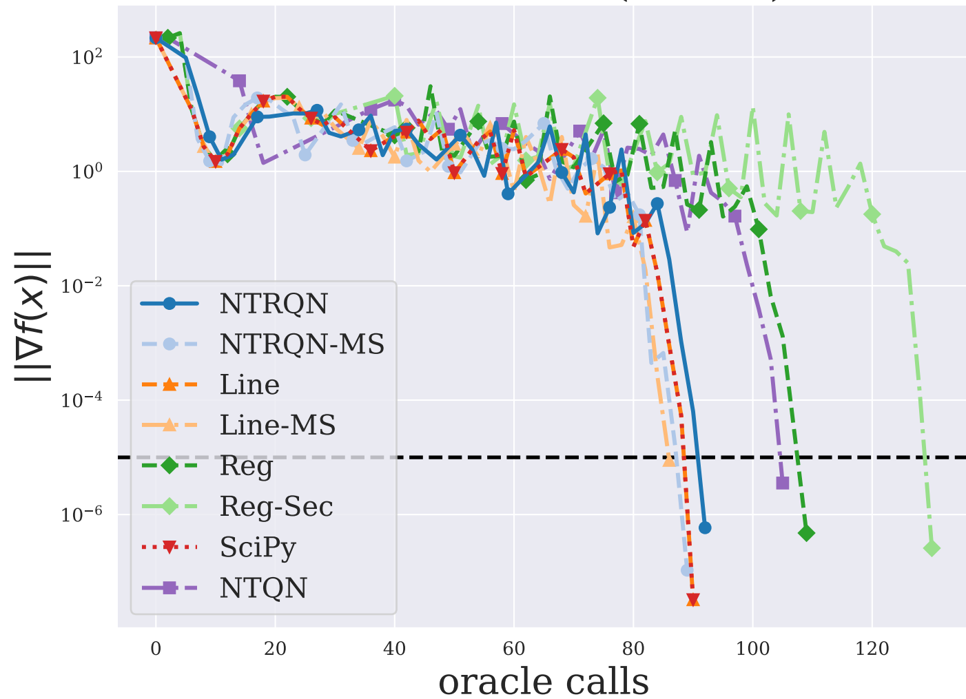
ROSENBR ( n = 2 )
